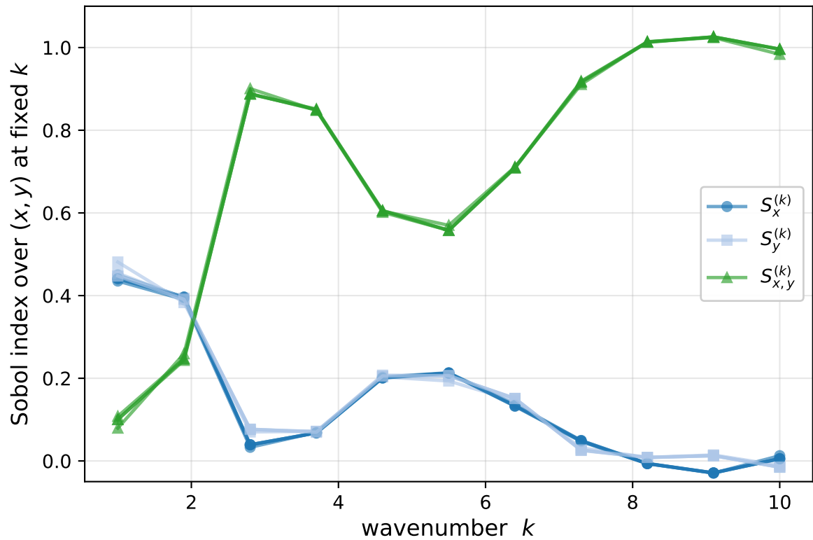
Spatial Sobol decomposition vs k — emergence of pair effect at high k
