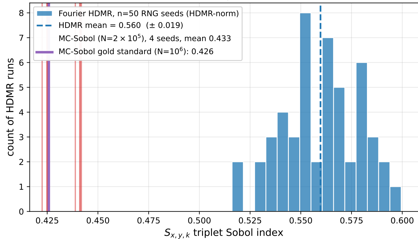
2D Helmholtz: distribution of triplet estimates across methods
