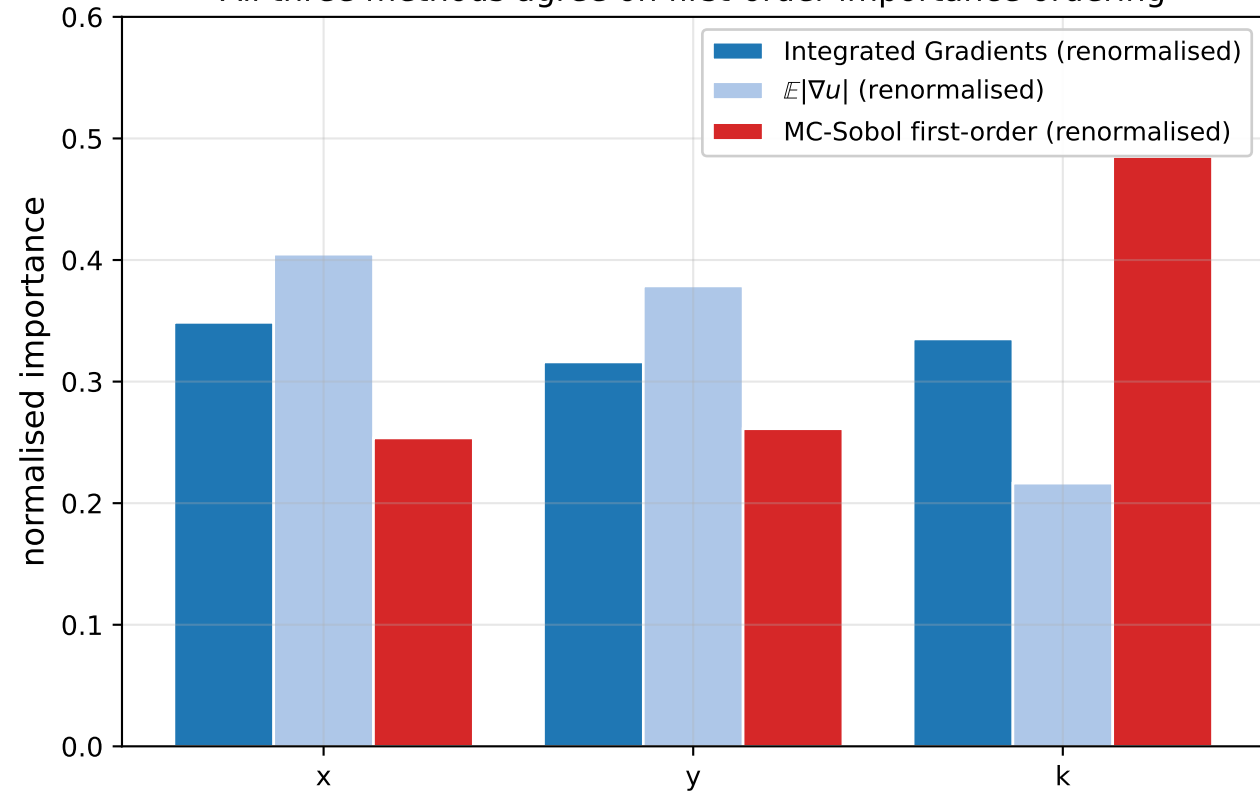
All three methods agree on first-order importance ordering
