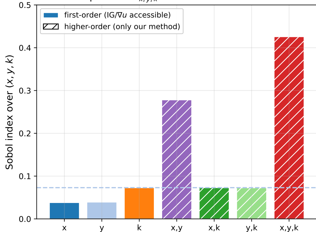
Full ANOVA decomposition: S_{x,y,k} = 0.43 is invisible to attribution methods
