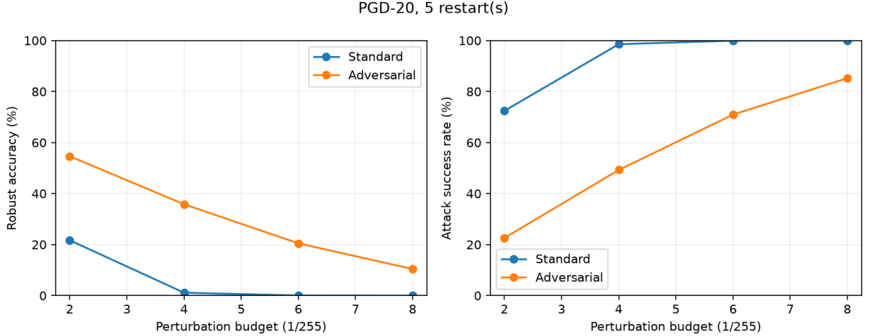
Figure 1: Measured robust accuracy and attack success rate. “Standard” denotes the clean continuation control. The figure is generated from the saved test measurements; the two ASR curves use their respective sets of clean-correct images as denominators.
