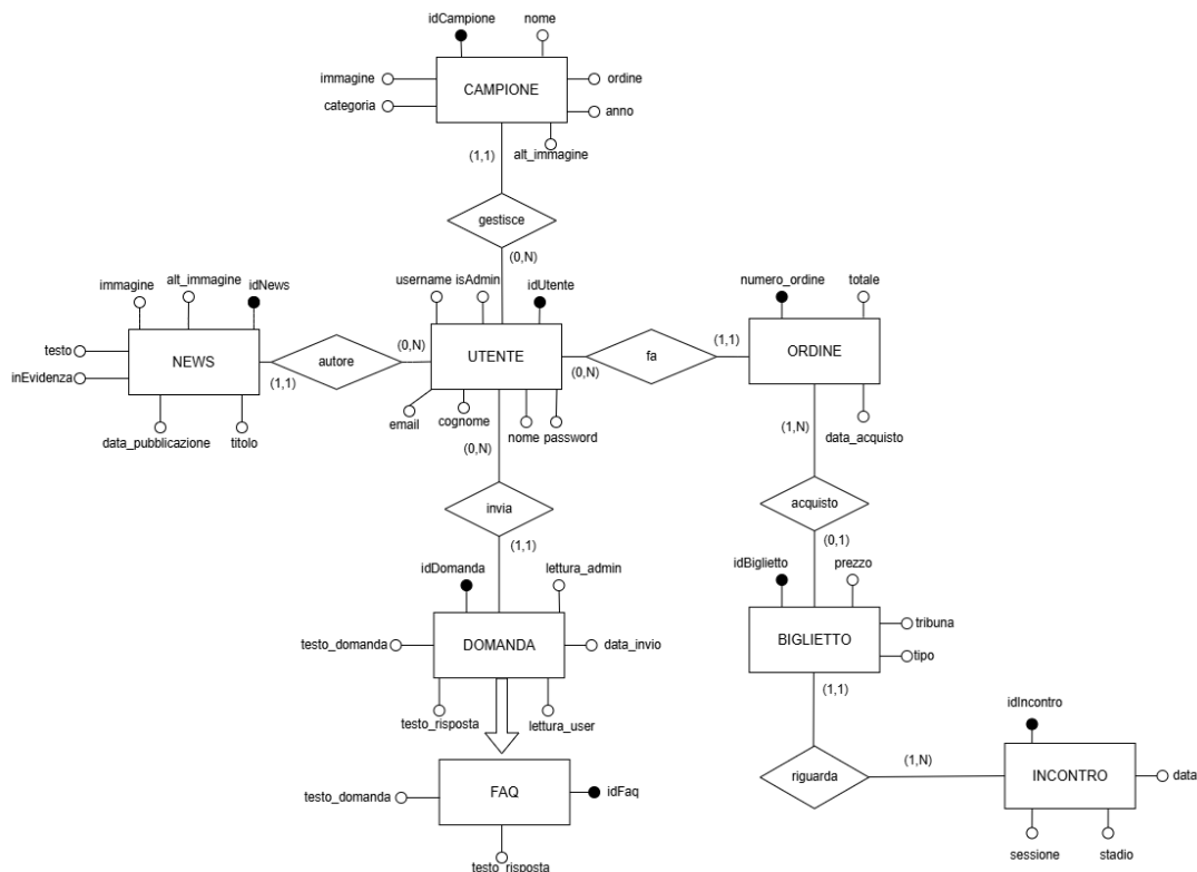
Figure 1: Schema E-R del database Patavium Open
