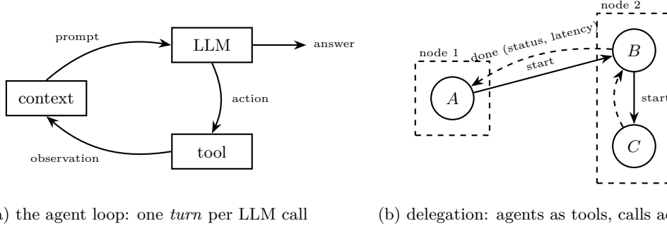
Figure 2.5: (a) The agent loop: each cycle through the LLM is one turn , appending the tool’s observation to the agent’s context. (b) Multi-agent delegation: once agents are tools, agent A calls agent B (possibly on another node), which calls C in turn, each call a start with a matching done (dashed) carrying status and latency. The result is a partially ordered event log with delegations as its cross-process edges.
