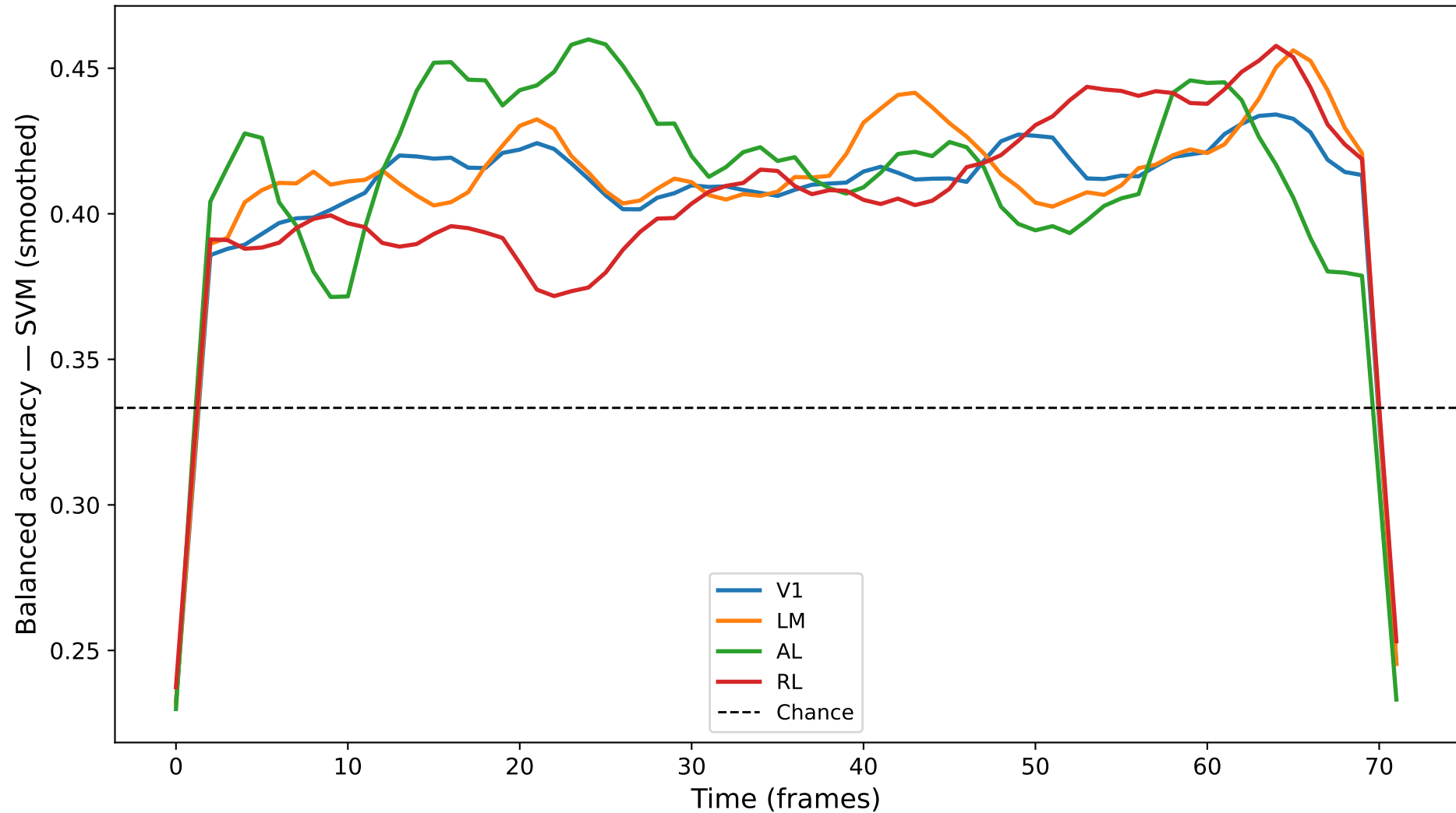
Q2: Smoothed decoding accuracy over time — SVM [w=5 frames]
