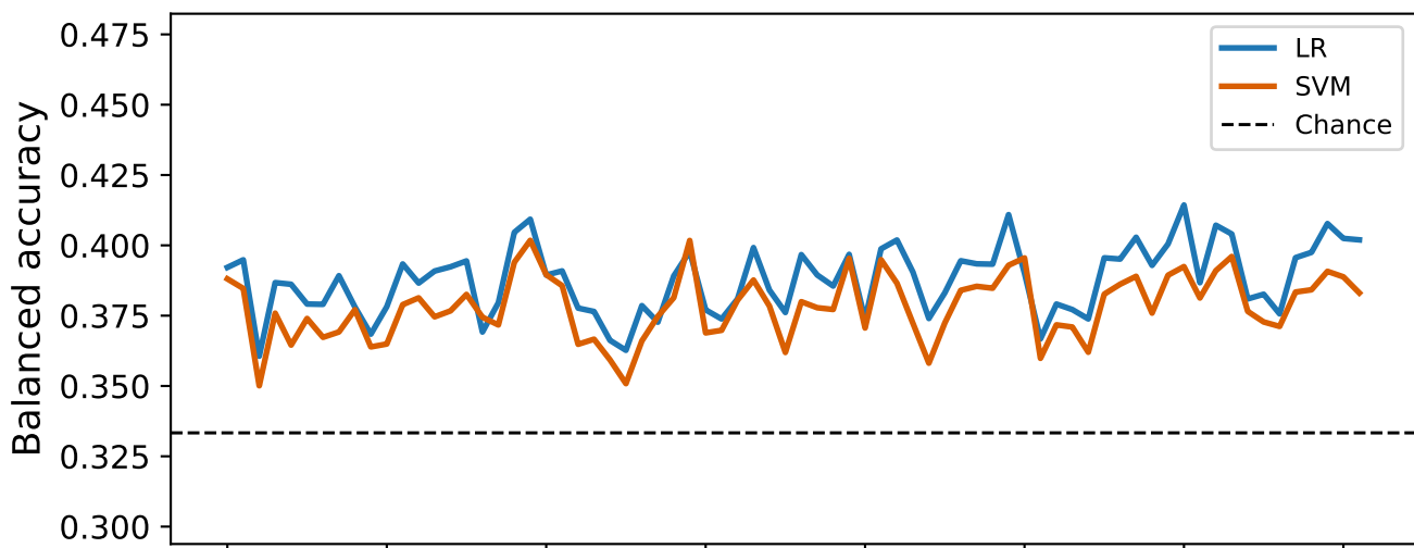
Q2: LR vs SVM accuracy over time [w=1 frame]
