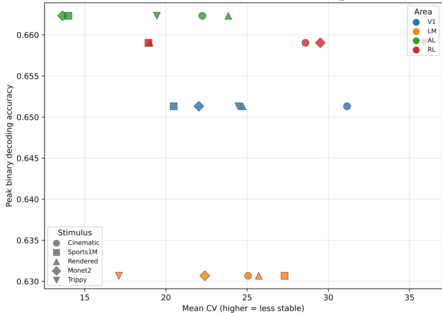
Q3.2: Stability vs Decodability — session 7_4
