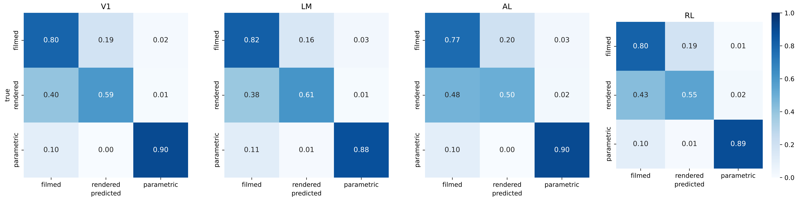
Q3: 3-class confusion (filmed/rendered/parametric) — session 5_6
