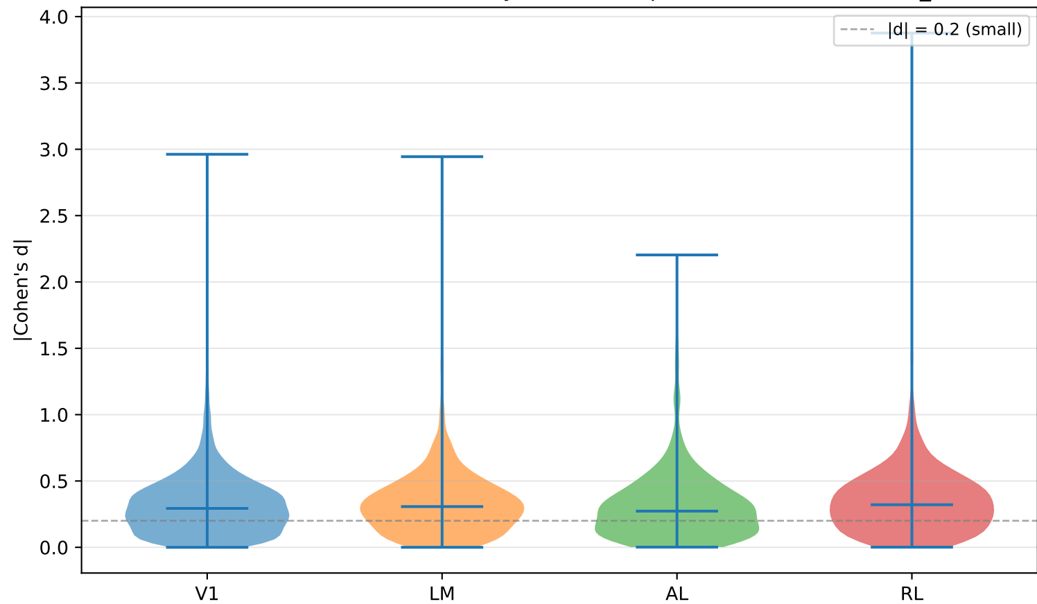
Q3: Per-neuron discriminability (natural vs parametric) — session 5_6
