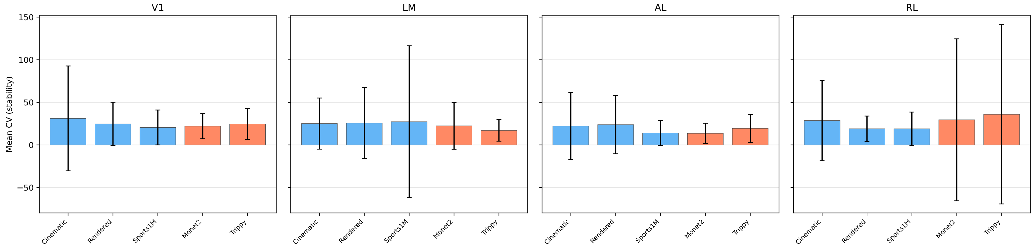
Q3.2: Firing-rate stability by stimulus type — session 7_4 (blue = natural, orange = parametric)
