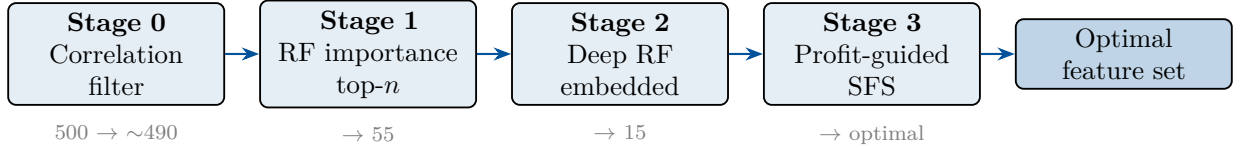
Figure 1: Four-stage profit-driven feature selection pipeline (Standard configuration).
