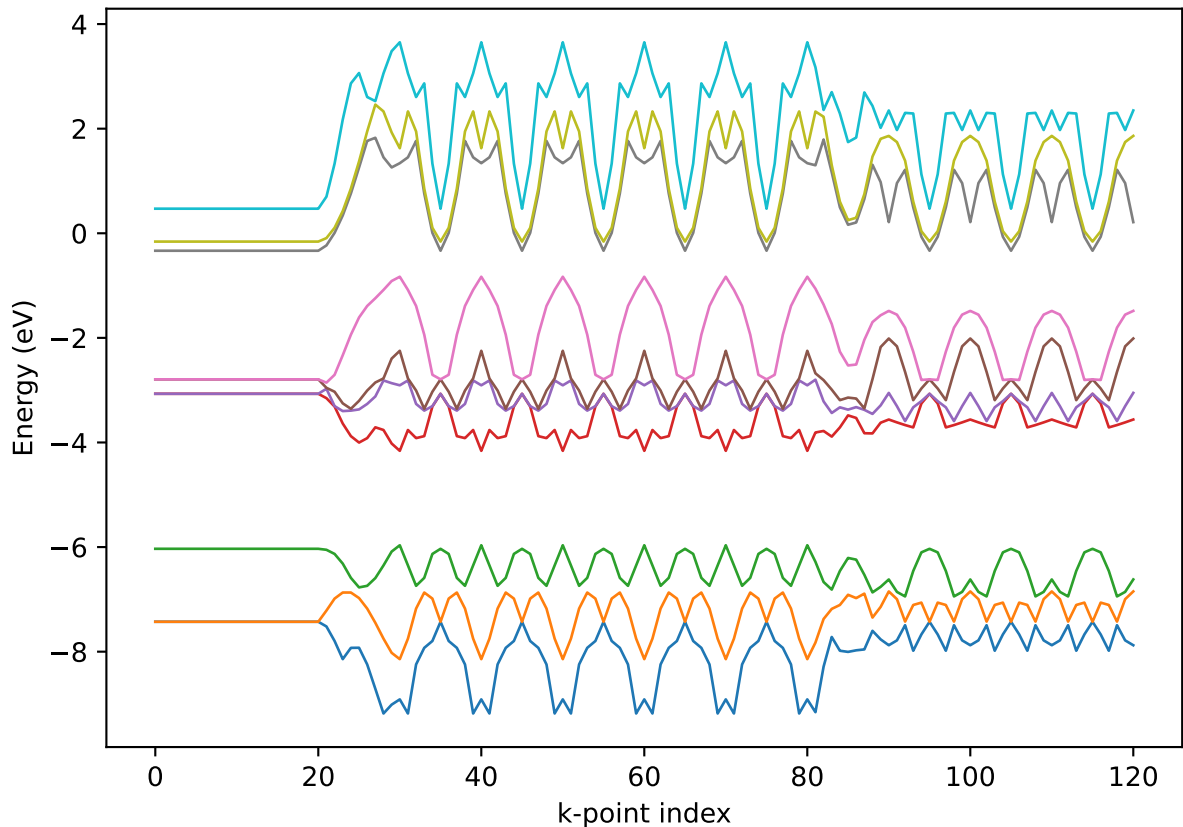
Bands from MoS2.bands.dat (nbnd=200, nks=121)
