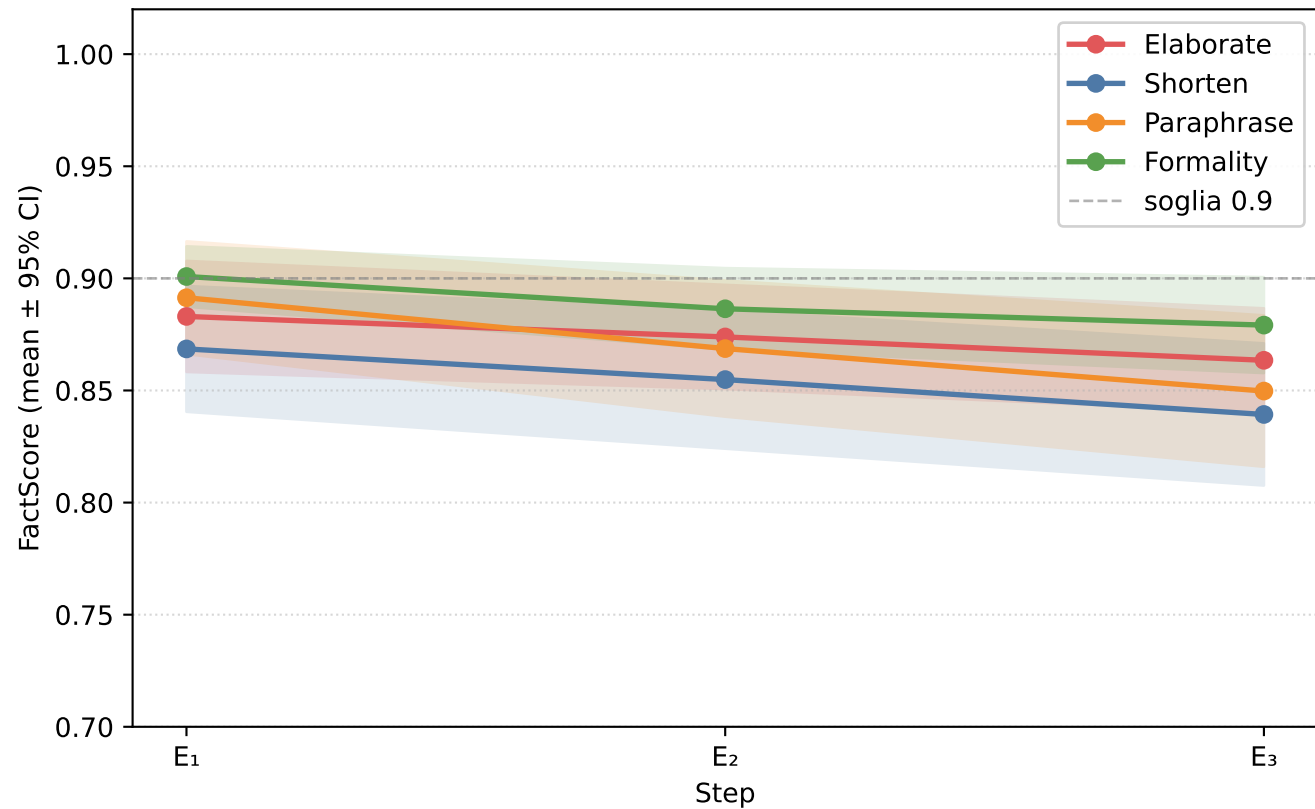
FactScore (w/ length penalty) — 25 qid
