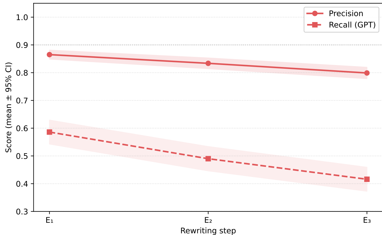
Precision vs Recall — Elaborate
