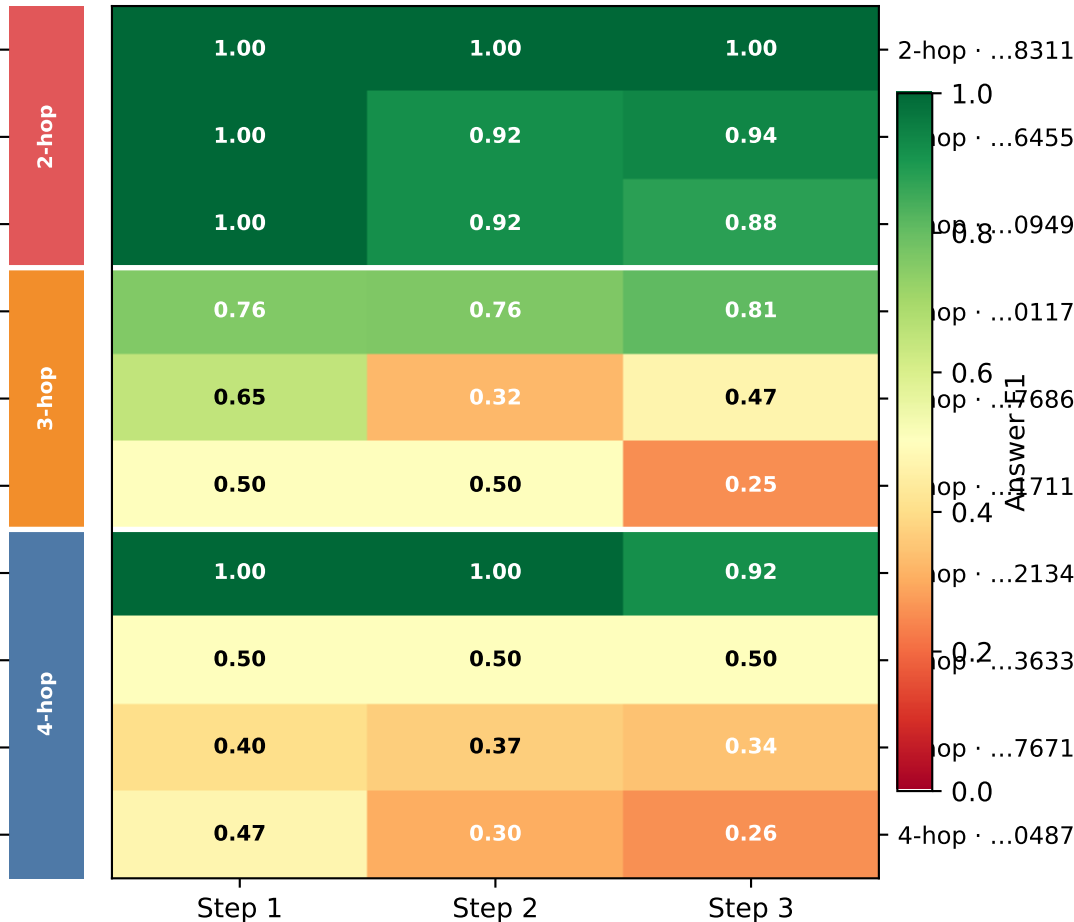
Answer F1 per question (mean across instructions and runs)
