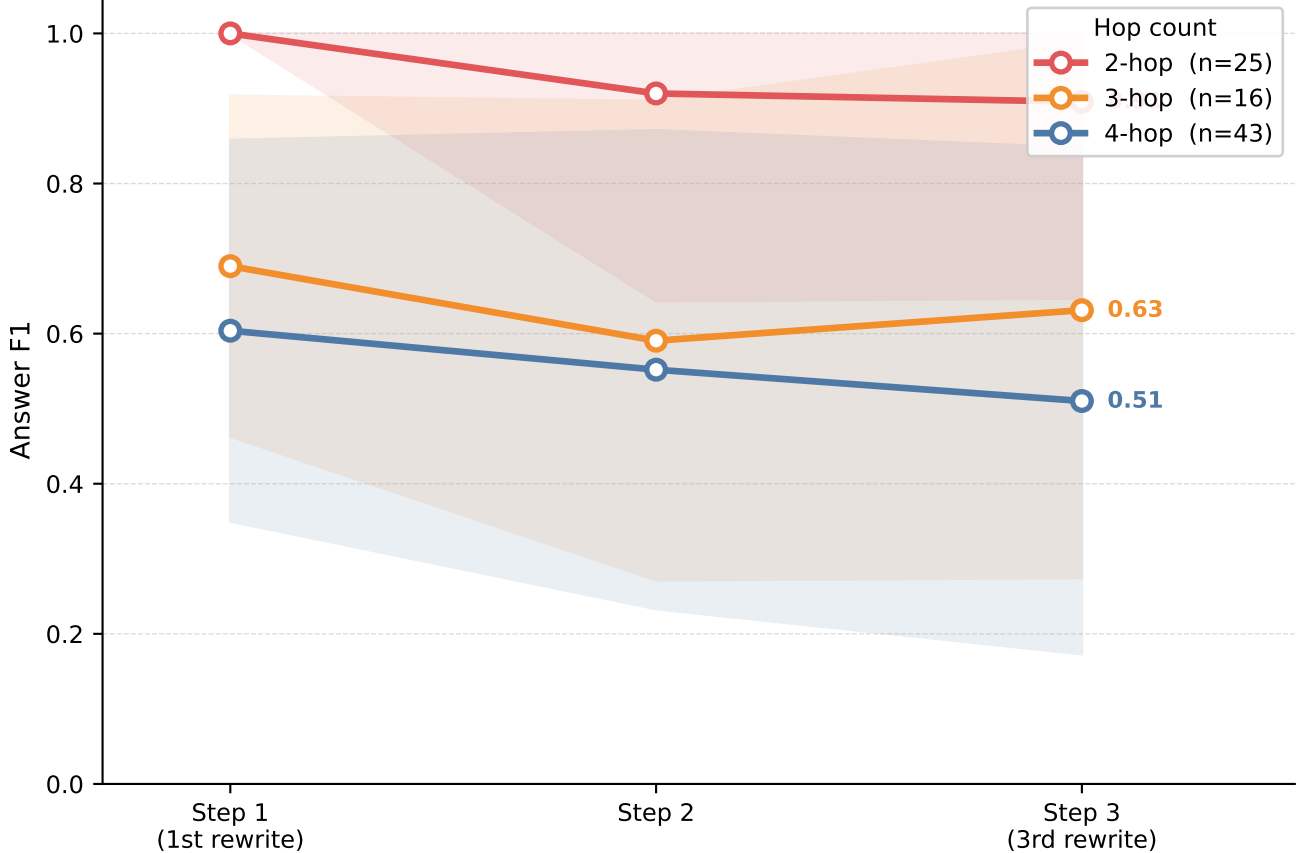
Answer F1 by question complexity (hop count)
