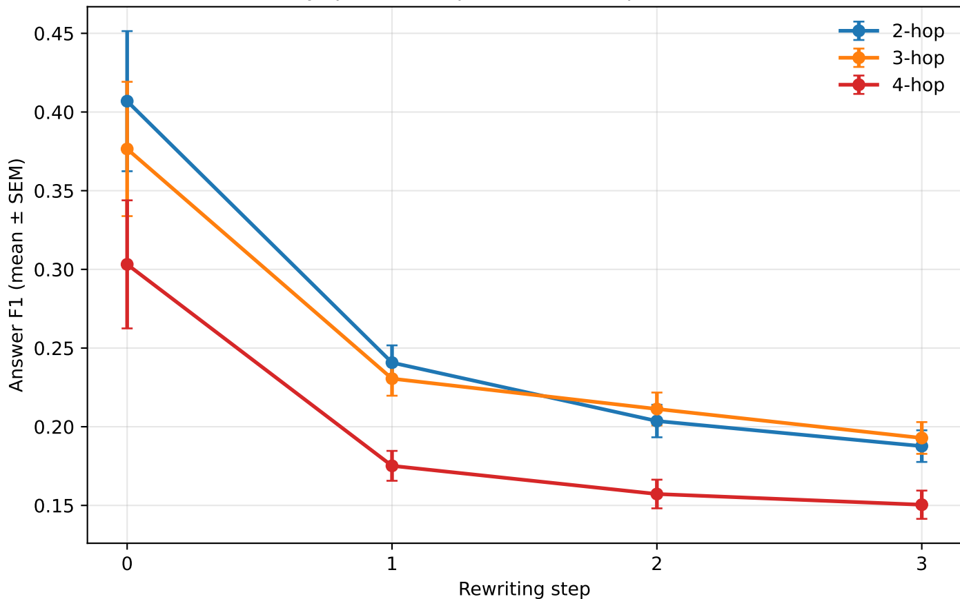
Answer F1 by question hop count — 300q (OLMo-3.1-32B, 4-bit)
