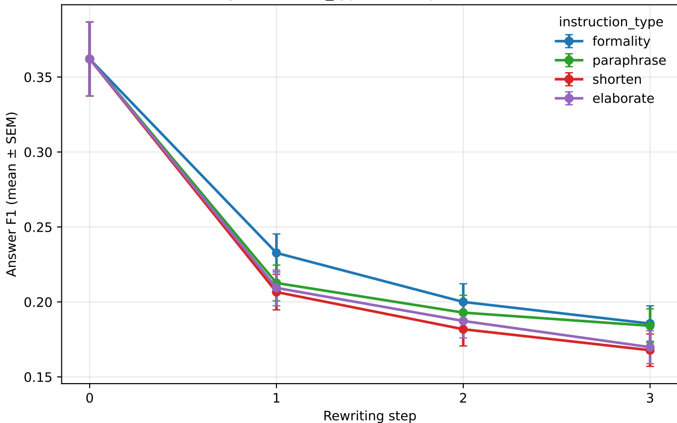
Answer F1 by instruction_type — 300q (OLMo-3.1-32B, 4-bit)
