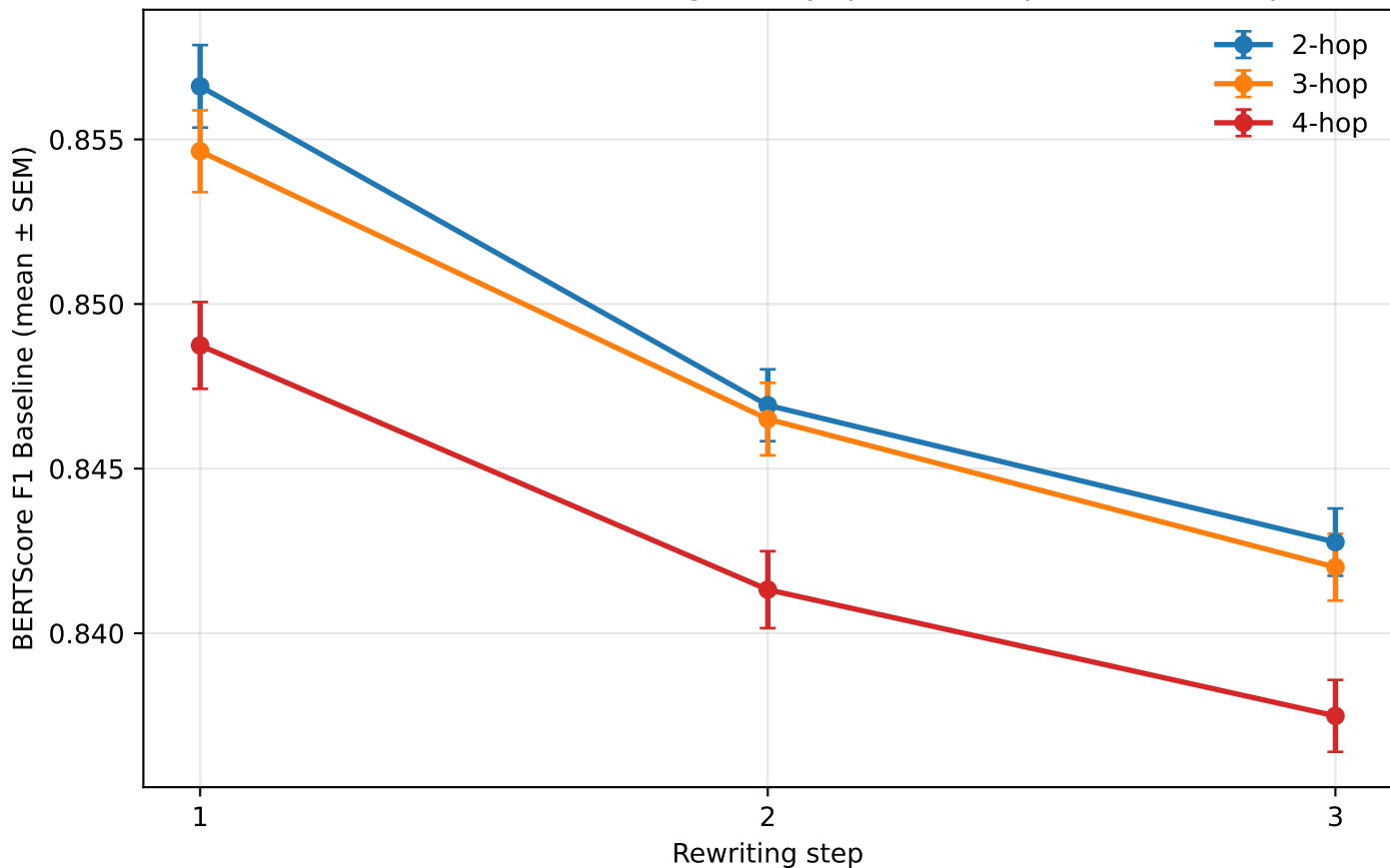
BERTScore Baseline (vs original) by question hop count — 300q
