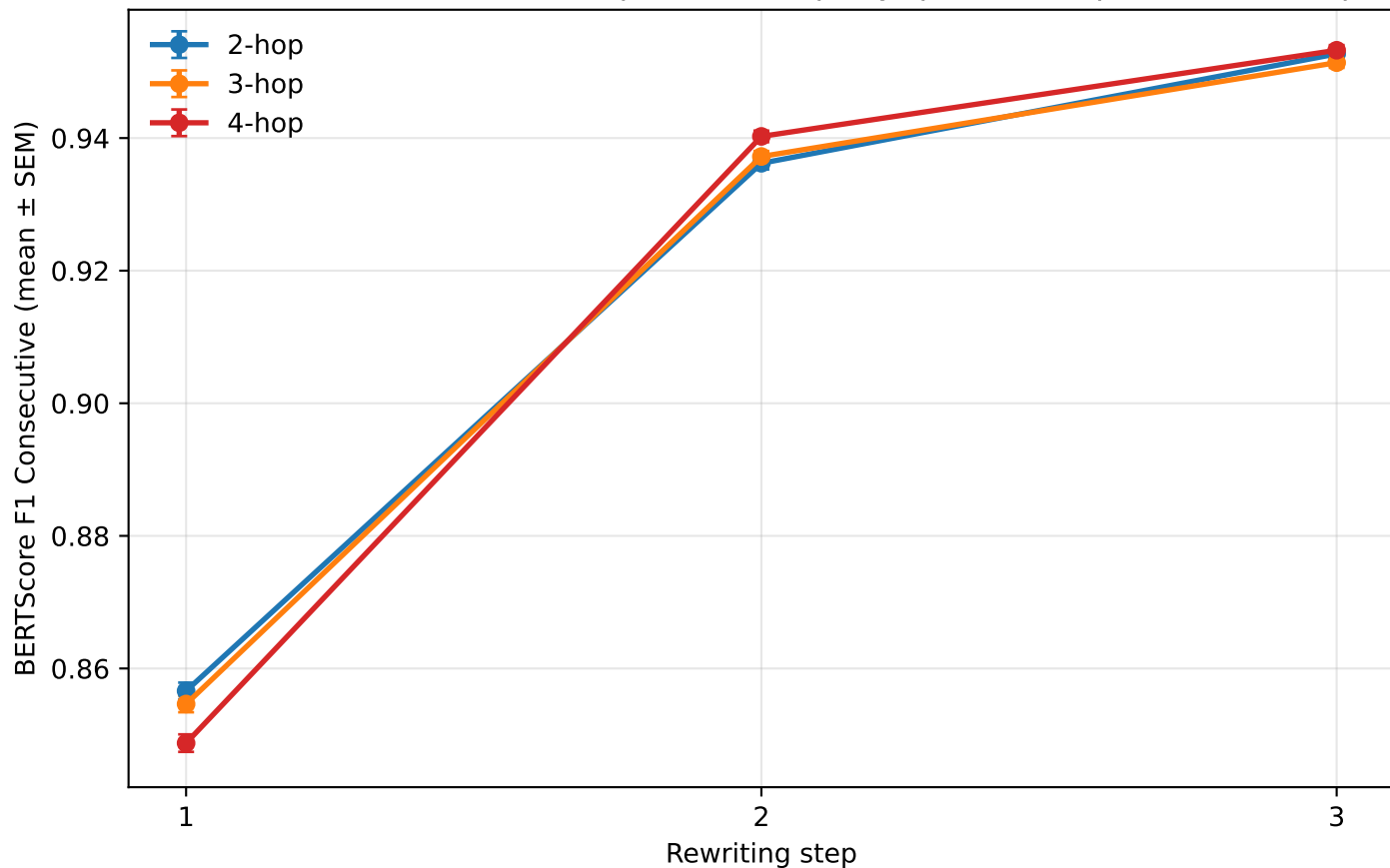
BERTScore Consecutive (vs previous step) by question hop count — 300q
