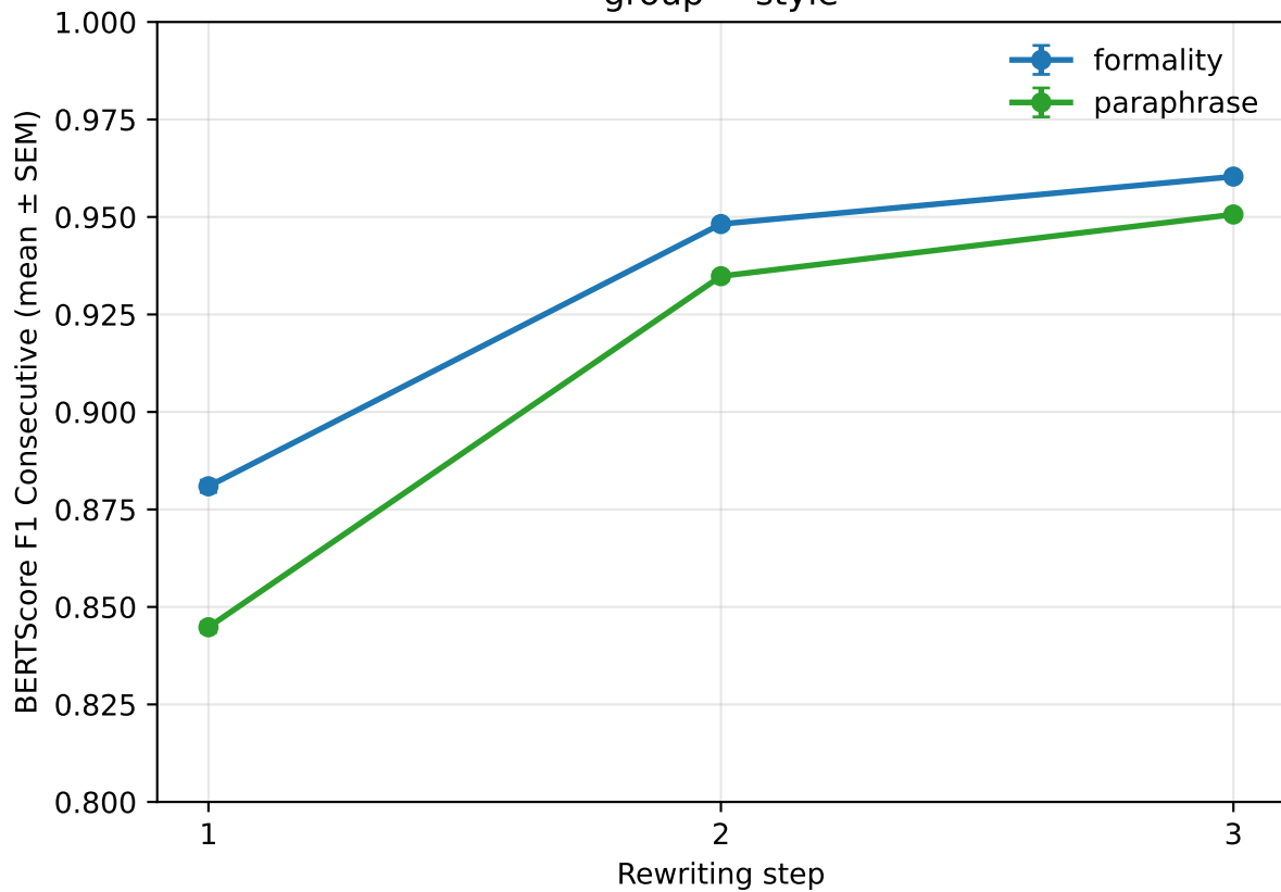
BERTScore Consecutive (vs previous step) across rewriting steps — 300q
