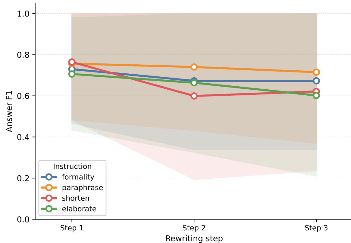
All answerable chains
