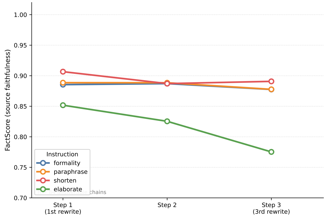
OpenFactScore by instruction type
