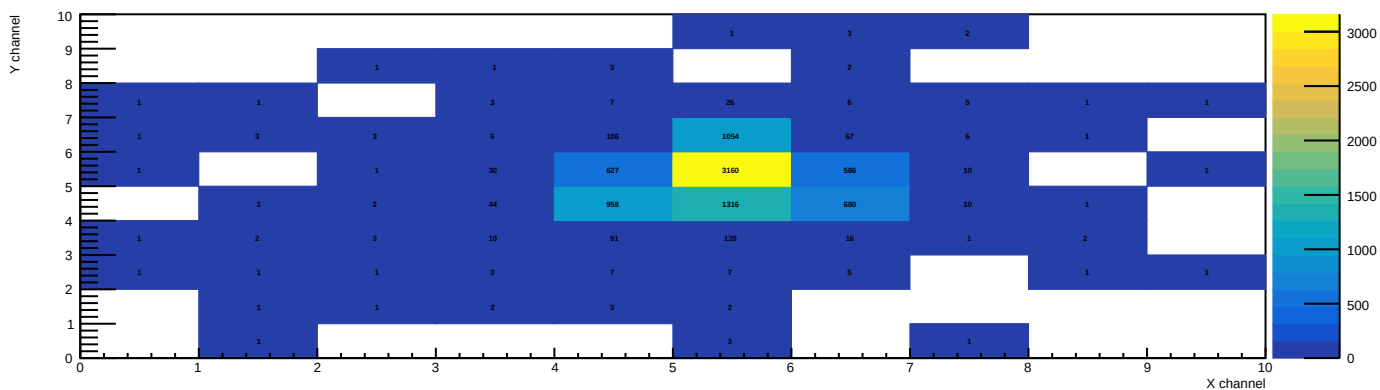
Hitmap of the second detector
