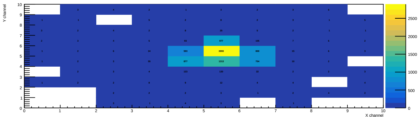
Hitmap of the first detector
