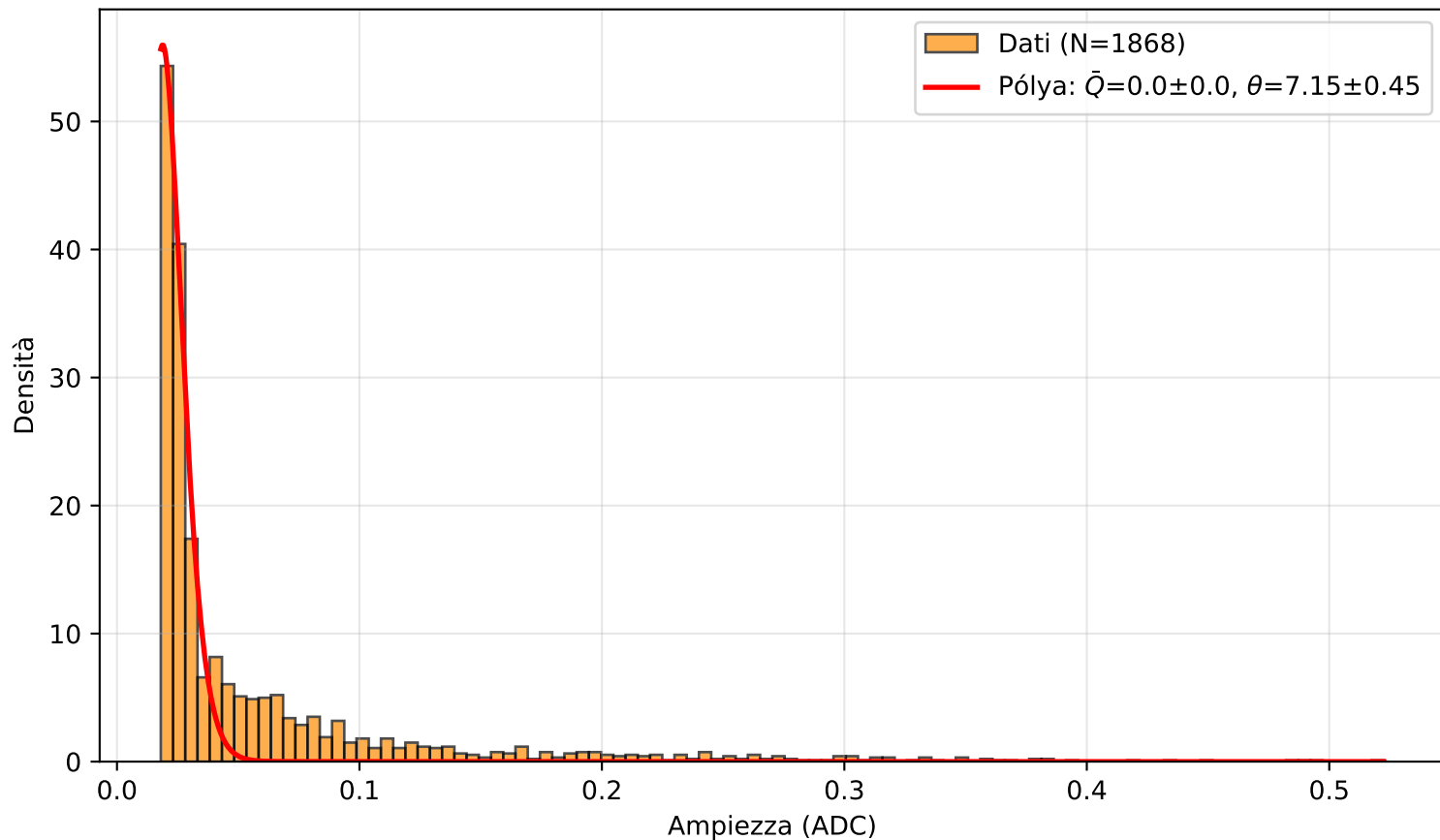
PICOSEC Detector 2 — Canale (4.0, 0.0)
