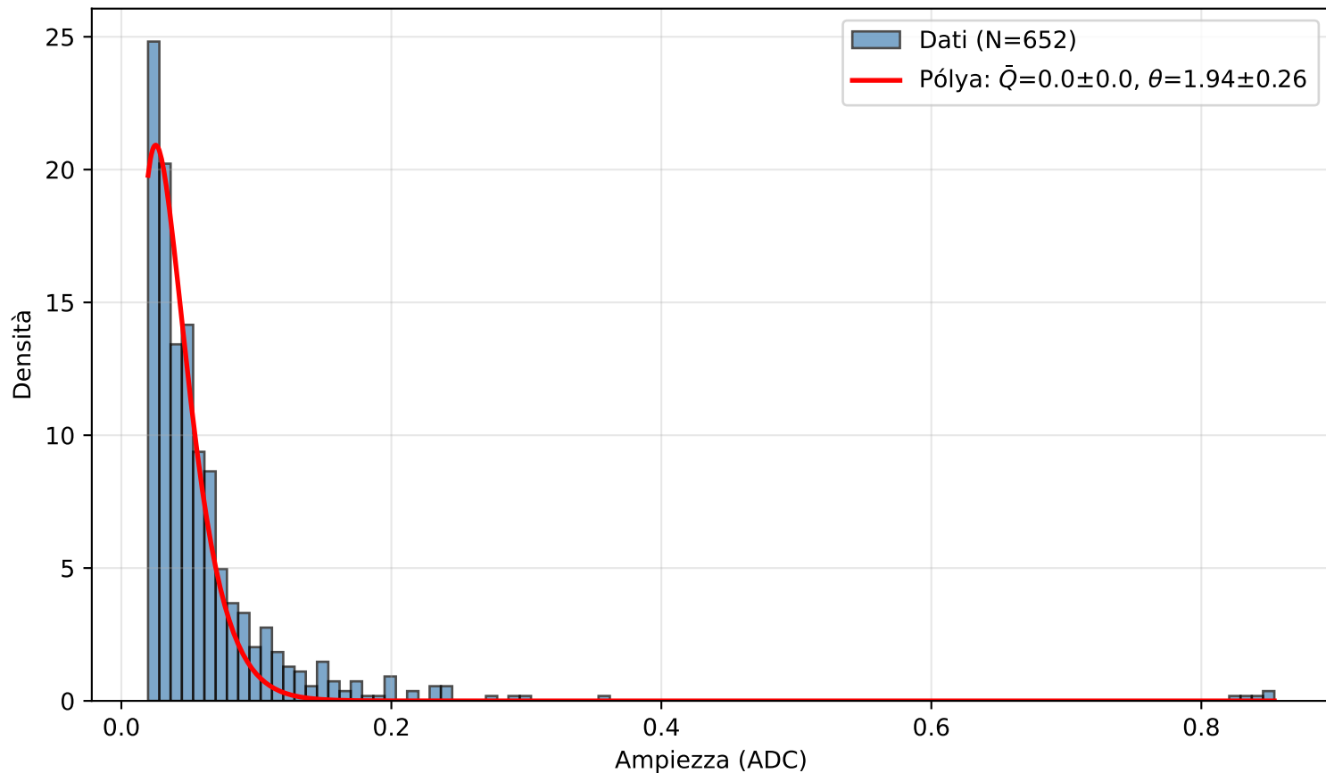
PICOSEC Detector 1 — Canale (7.0, 3.0)
