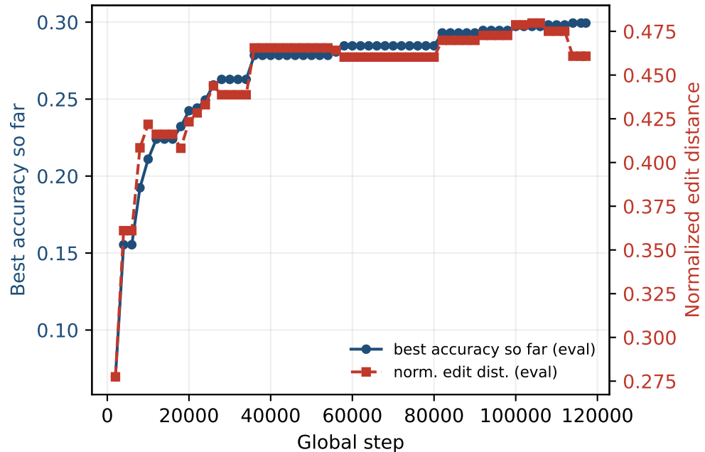
Held-out evaluation (best-so-far) (150k, 25 epochs)
