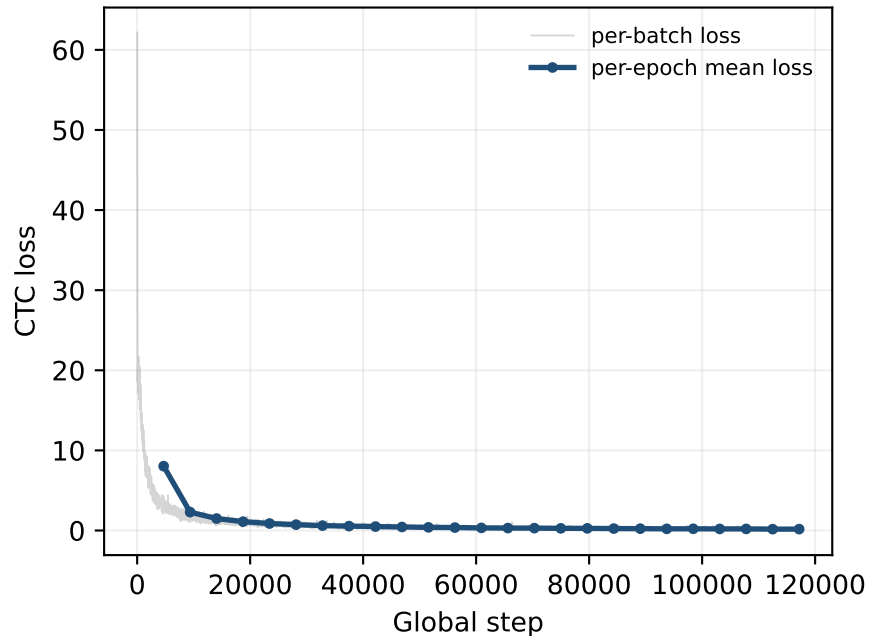
Training loss (150k, 25 epochs)
