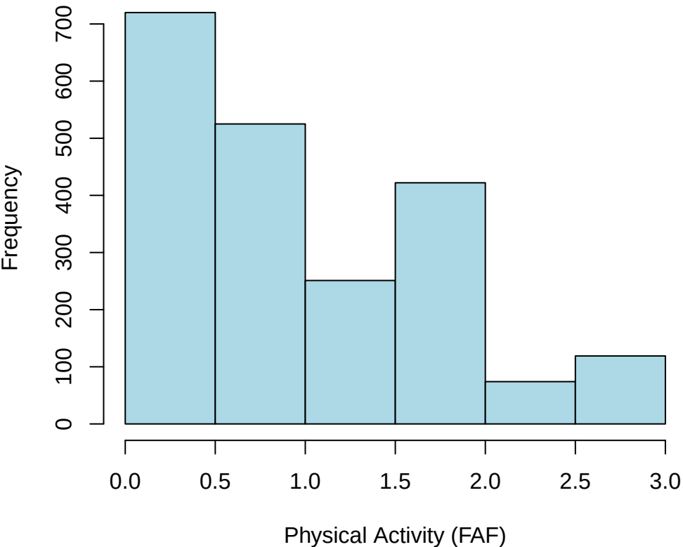
Histogram of Physical Activity (FAF)
