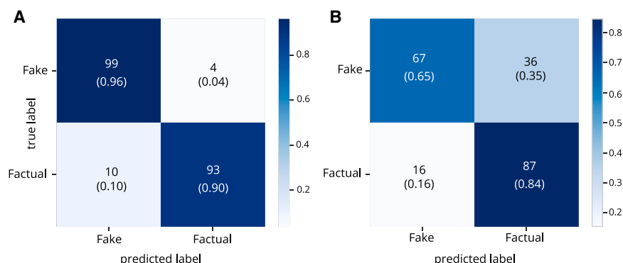
Figure 3. Confusion matrix for the XGBoost model
