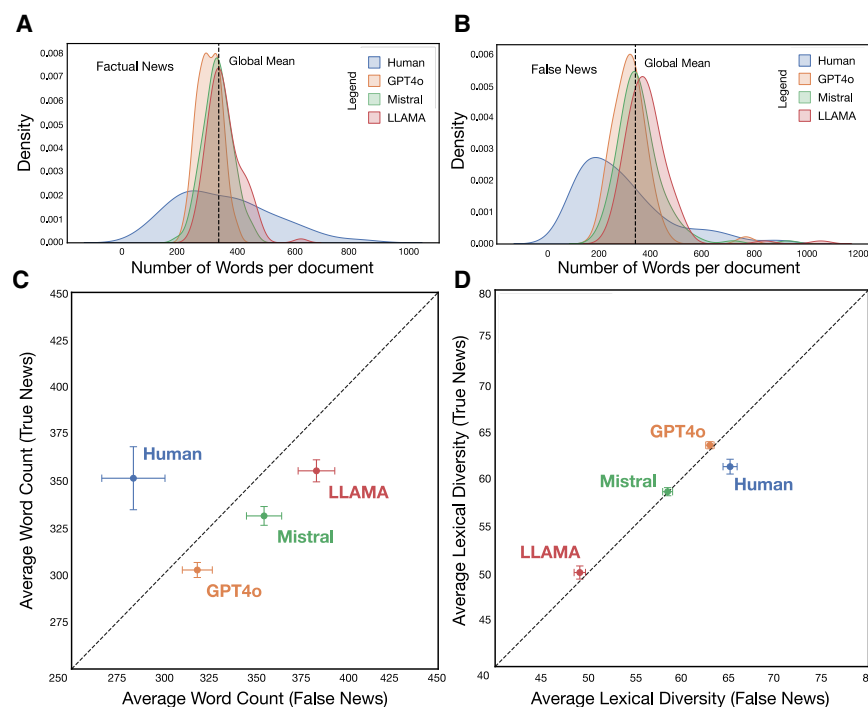
Figure 1. Descriptive comparison between the documents produced by humans and LLMs
