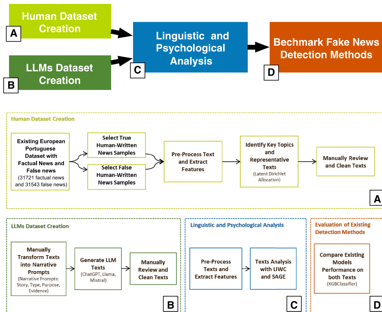
Figure 4. Illustration of the four stages of the methodology pipeline
