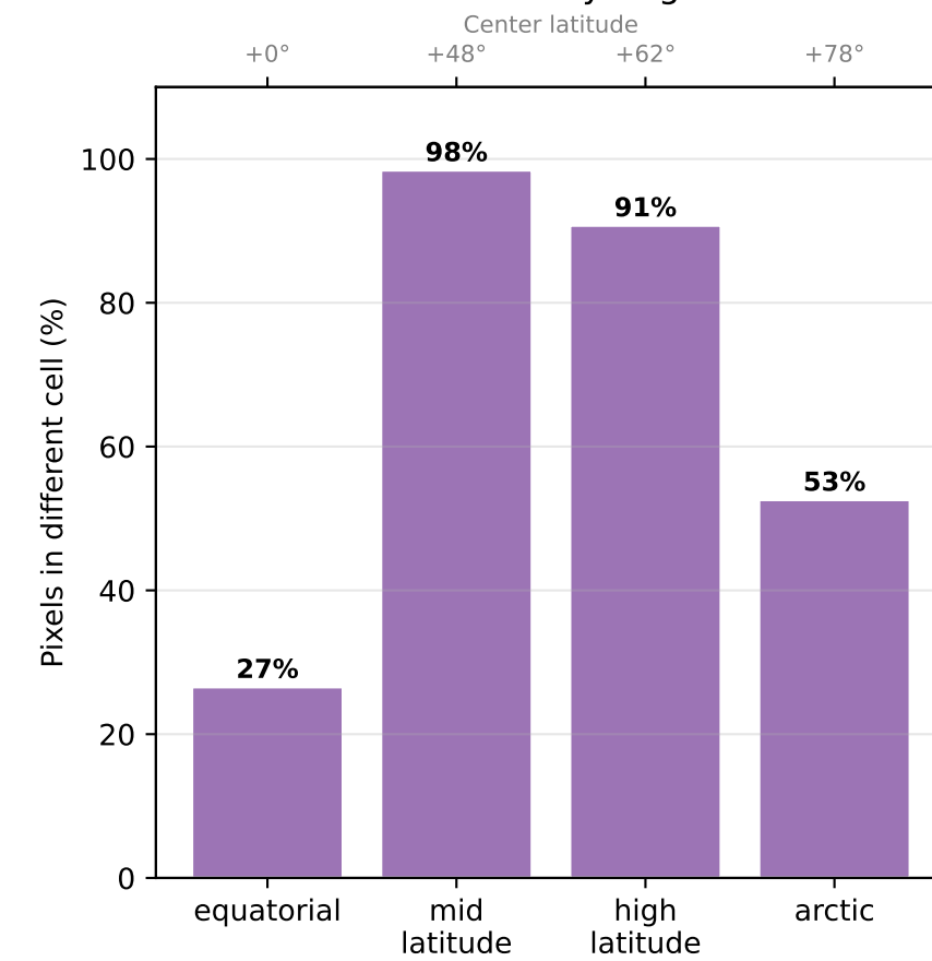
Sphere vs WGS84 Indexing Difference by Region
