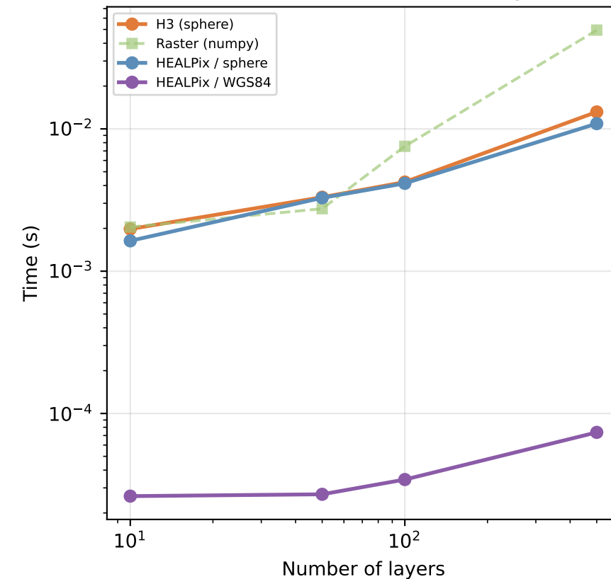
Raster Benchmark — Timing
