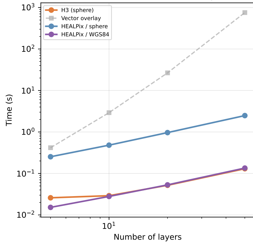
Vector Benchmark — Timing
