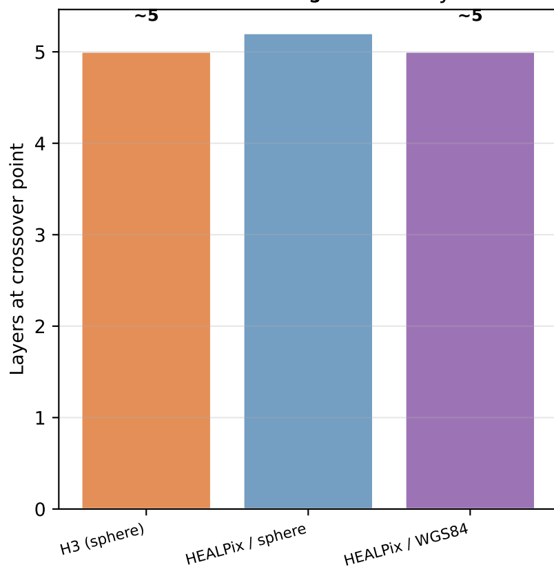
Crossover: DGGS becomes faster than vector overlay
