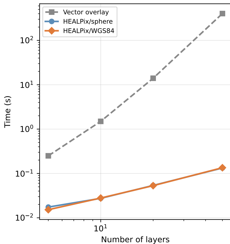
Vector Benchmark
