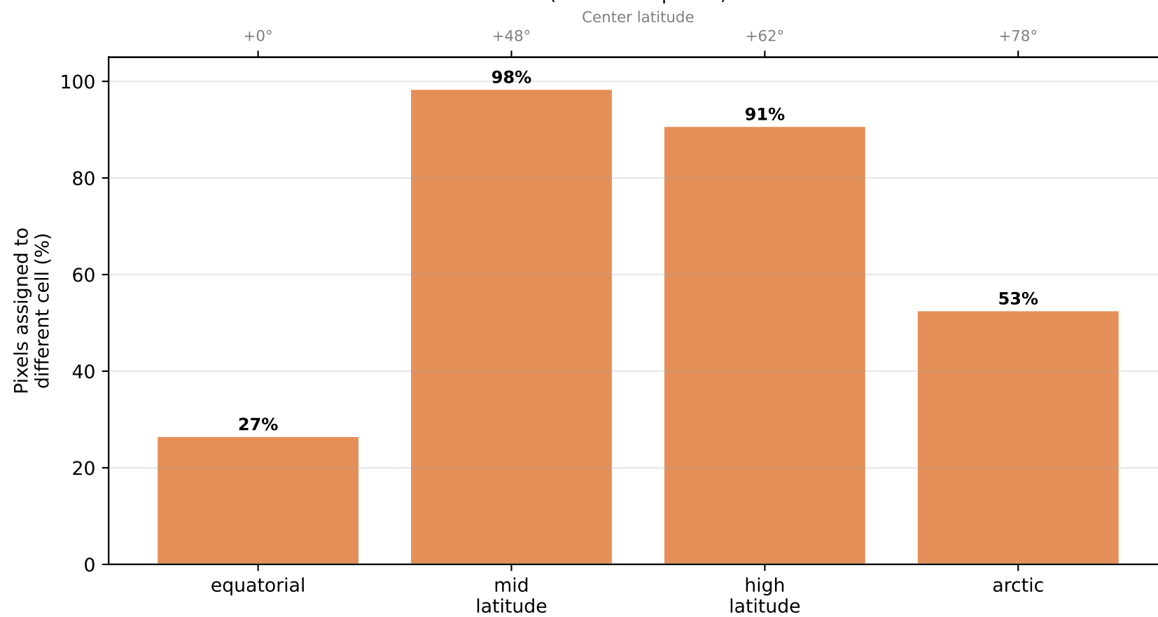
Sphere vs WGS84 Indexing Difference by Region (HEALPix depth=9)
