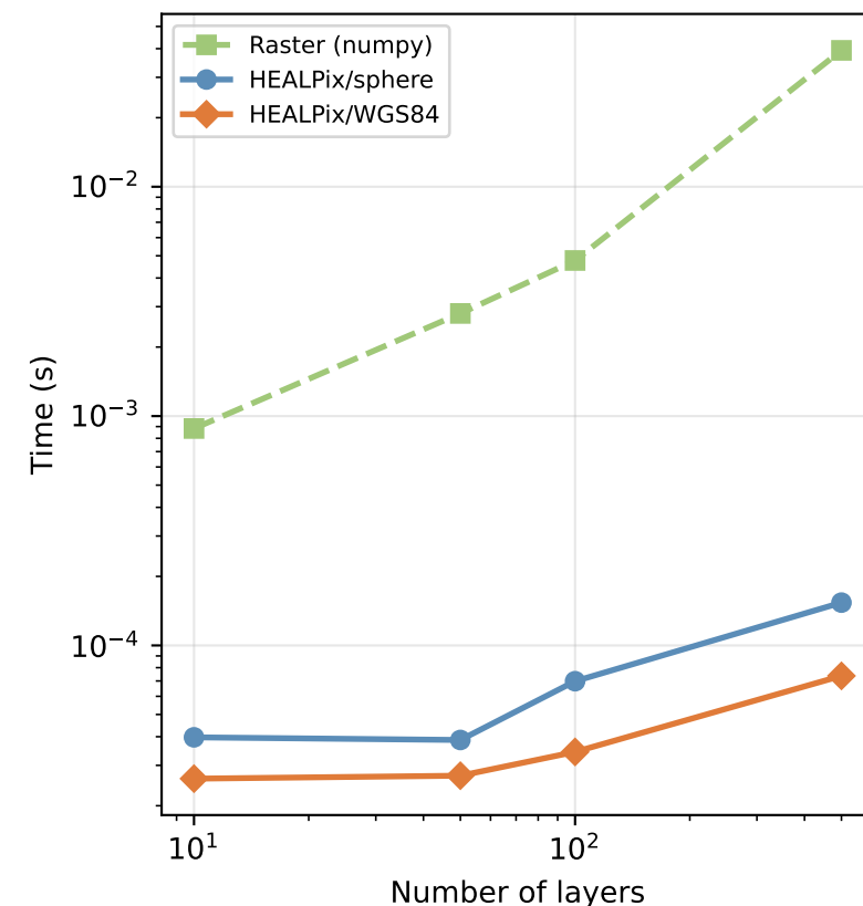
Raster Benchmark
