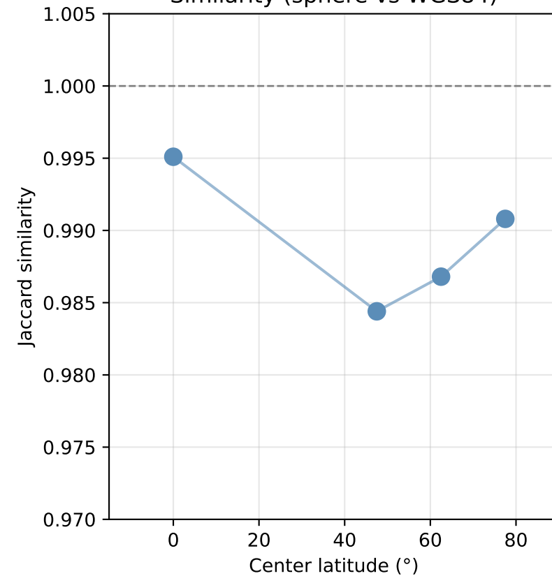
Polygon Coverage Similarity (sphere vs WGS84)
