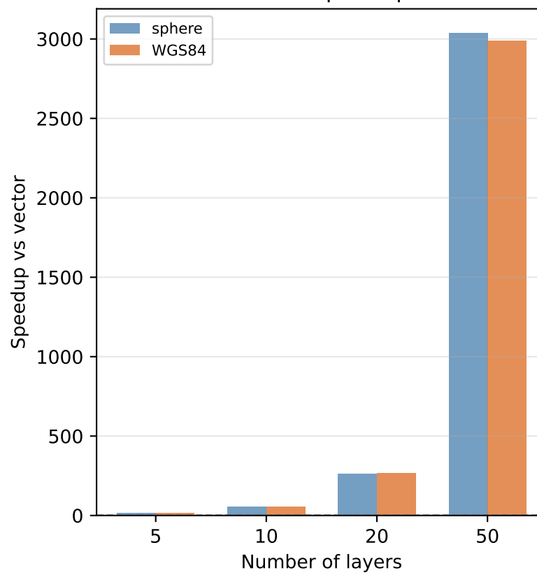
Vector Speedup
