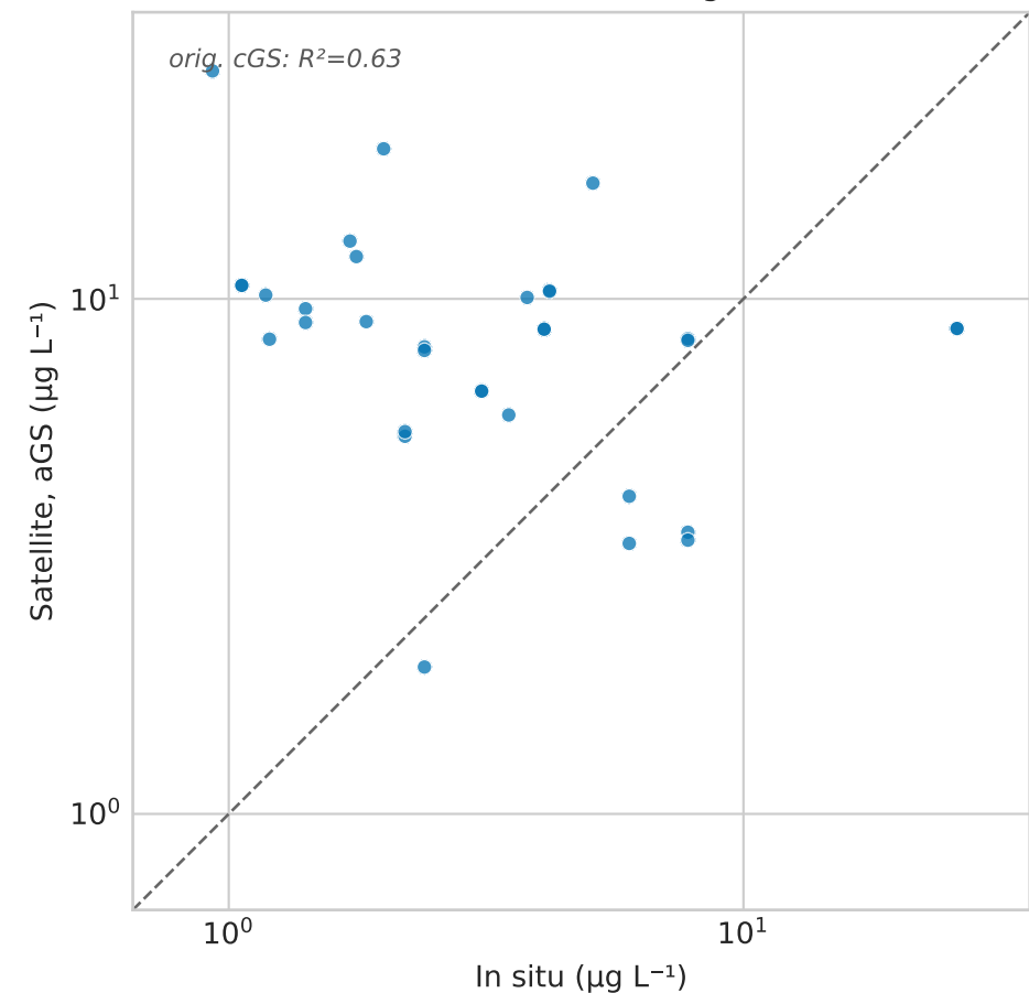
Parameter-dependent retrieval accuracy in the Westerschelde (open-source chains) vs the original study
