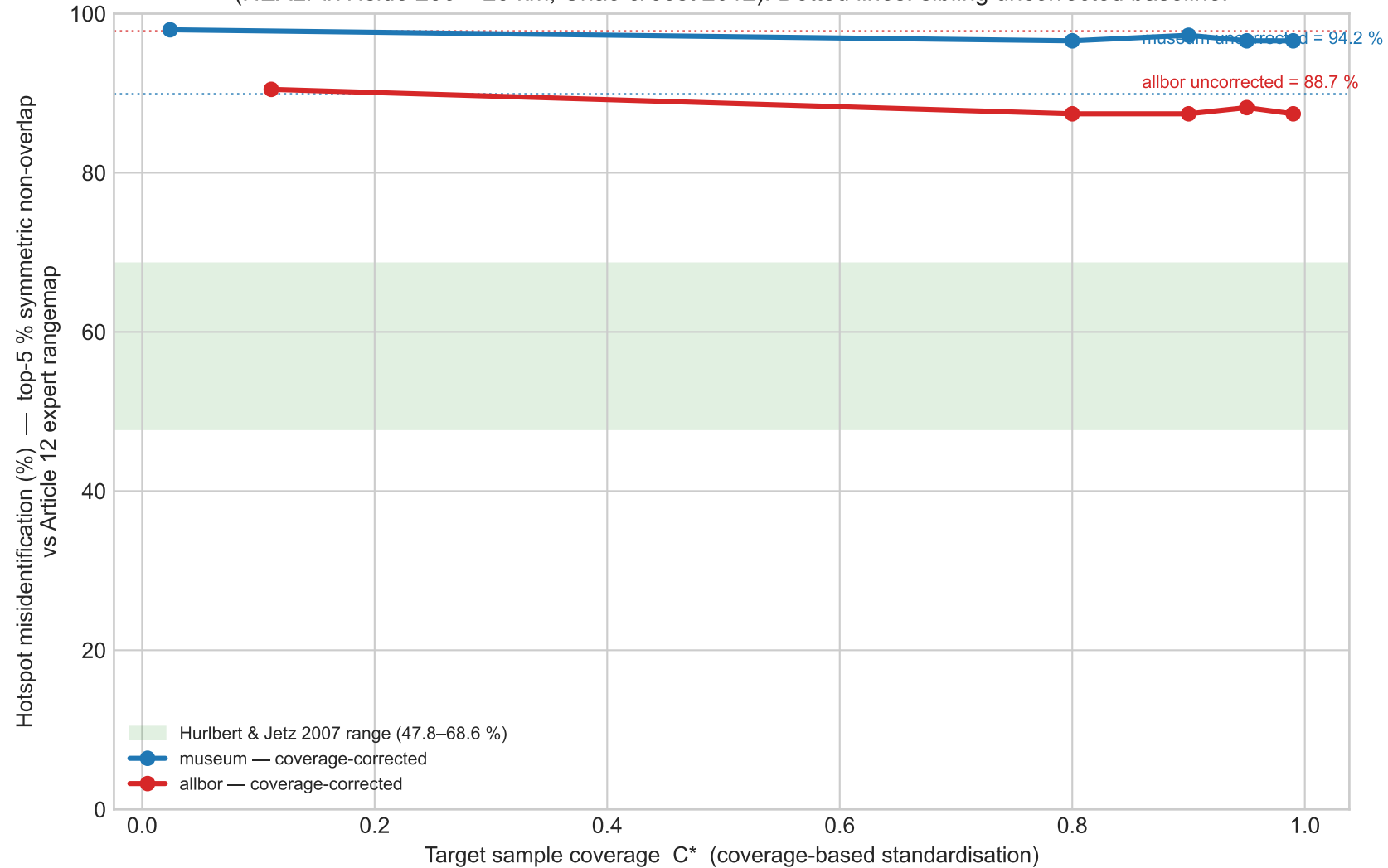
Coverage-based effort correction of Iberian-bird richness hotspots (HEALPix Nside 256 \approx 25 km; Chao & Jost 2012). Dotted lines: sibling uncorrected baseline.
