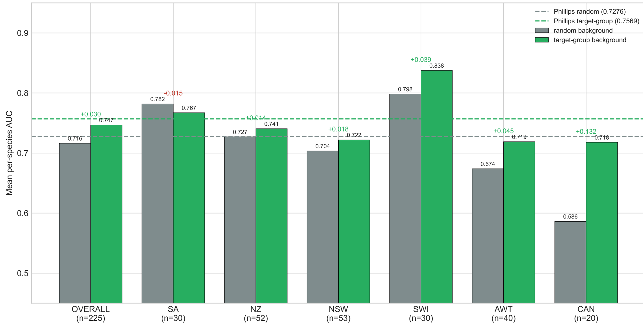
Reproduction (Arm A): target-group background improves MaxEnt AUC Elith et al. 2006 NCEAS benchmark — elapid MaxEnt — vs Phillips 2009 Table 2
