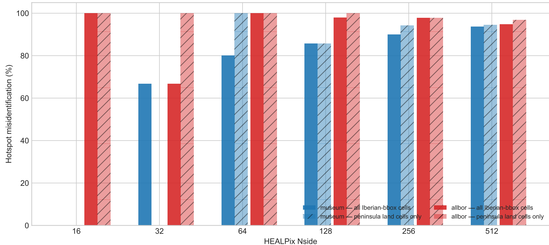
Test 1 — Land mask sensitivity all Iberian-bbox cells (solid) vs peninsula-only (hatched)
