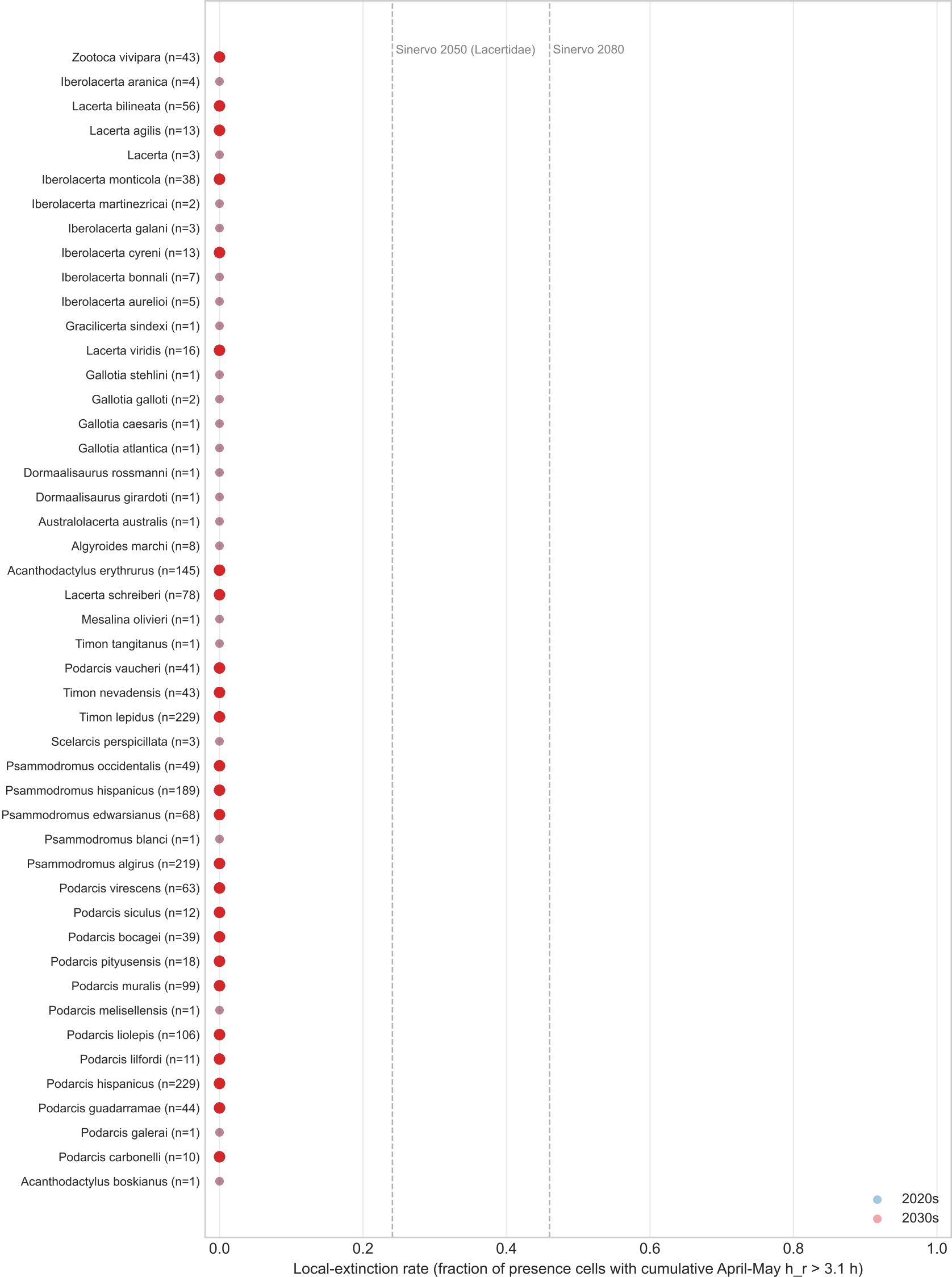
Iberian Lacertidae — local-extinction rate per species (DestinE SSP3-7.0) family-wide: 0.0% (2020s) | 0.0% (2030s)
