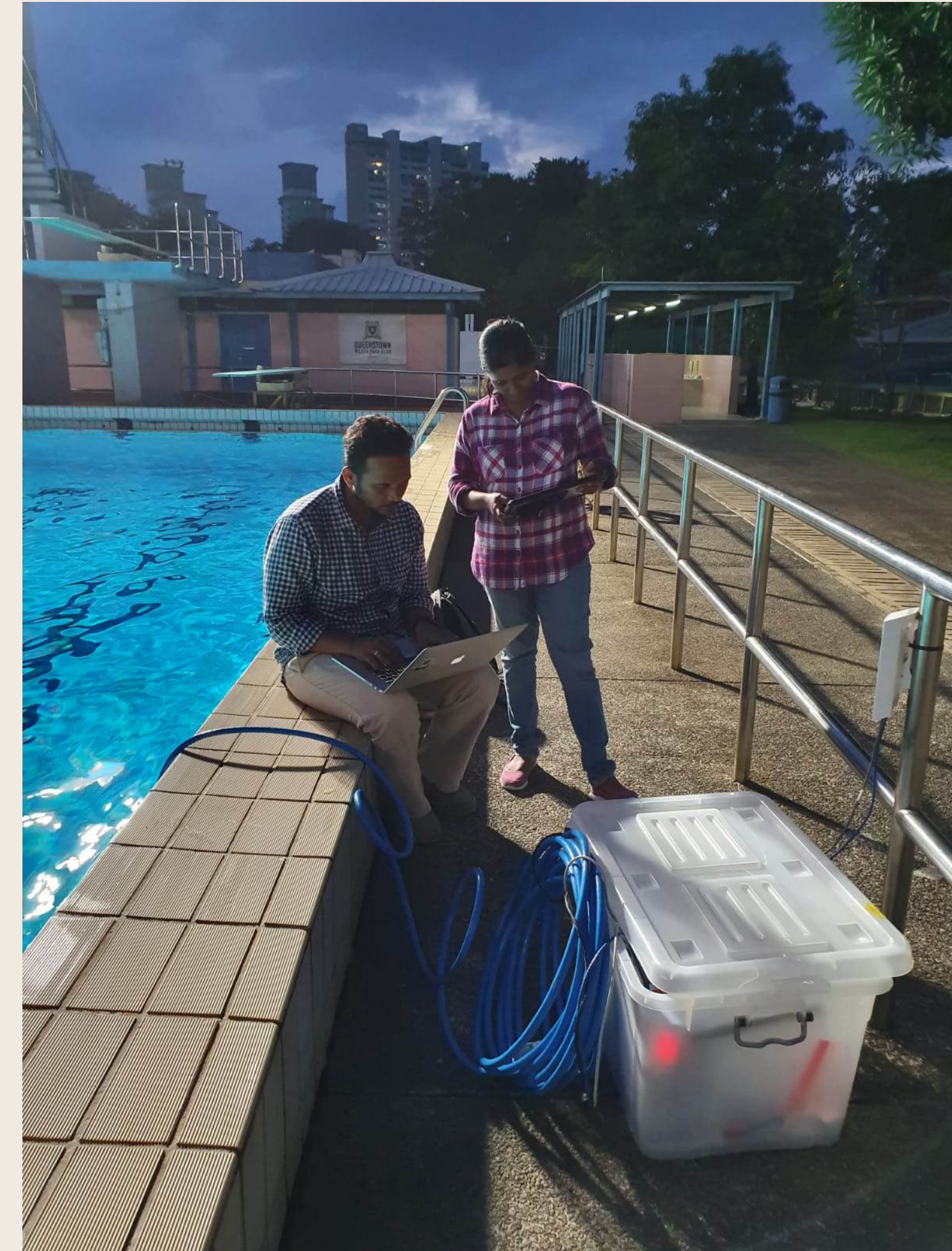
On-field testing of underwater asset at a swimming pool
