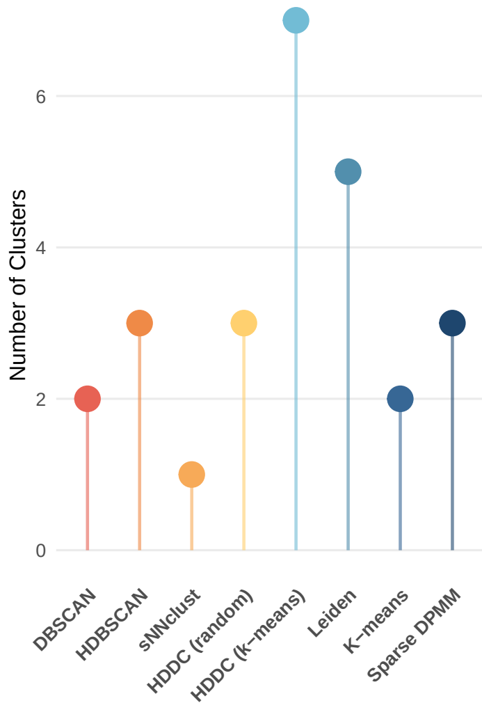
(a) Estimated Clusters
