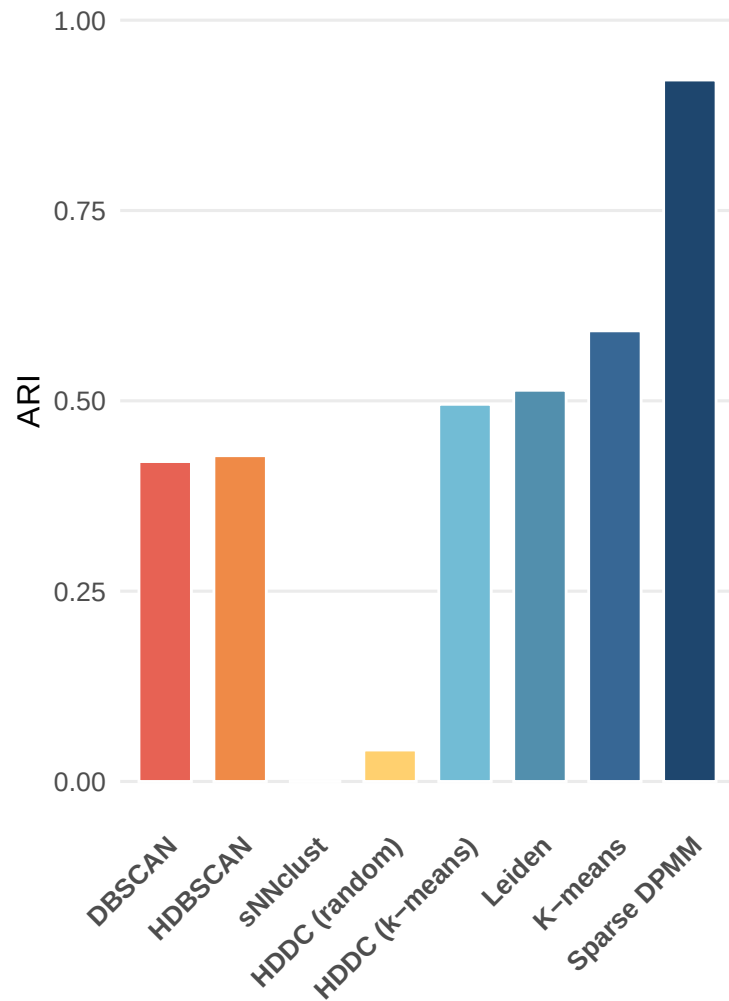
(b) ARI Score
