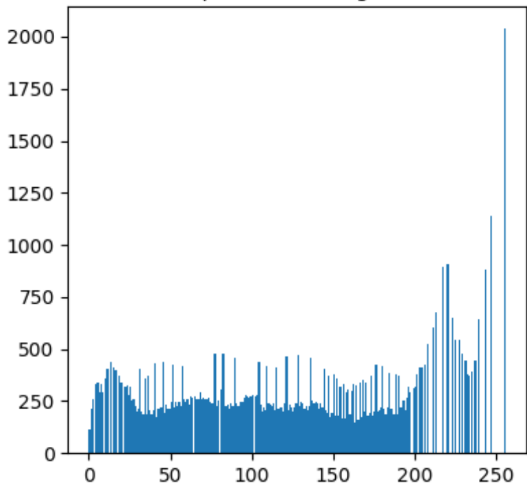
Equalized Histogram
