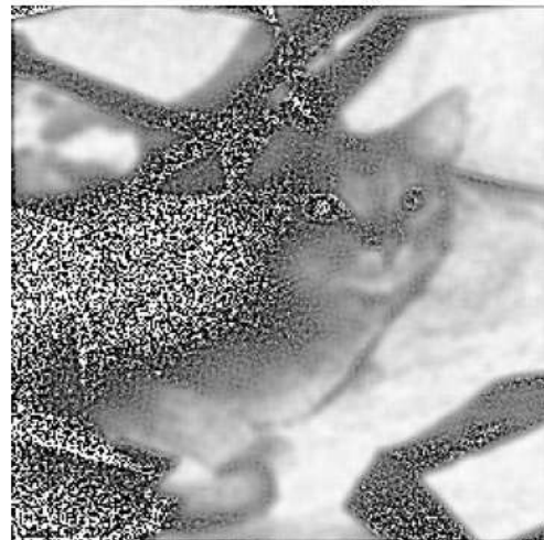
Wiener Filtering
