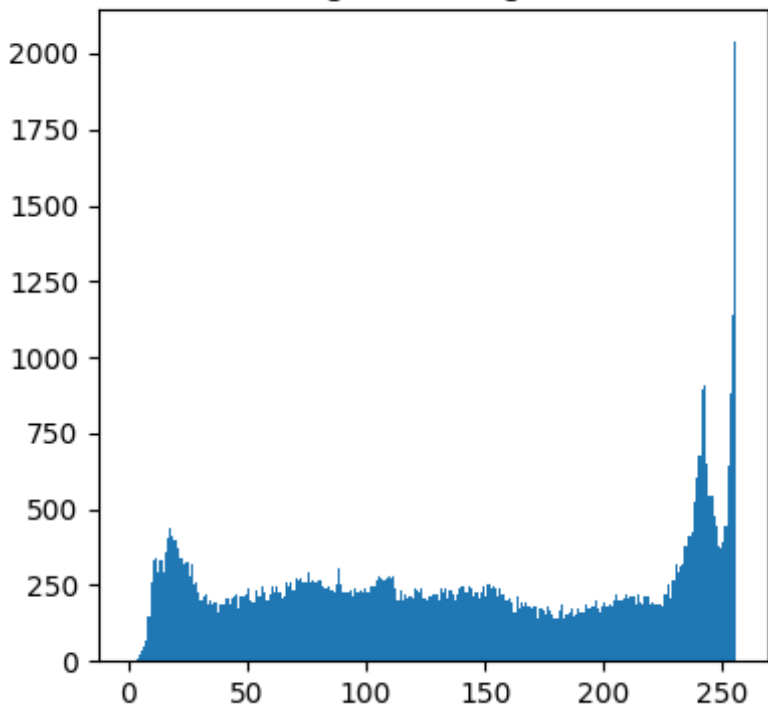
Original Histogram
