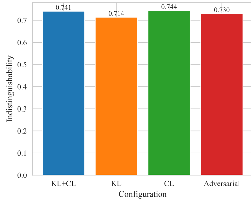
Loss Configurations: Indistinguishability
