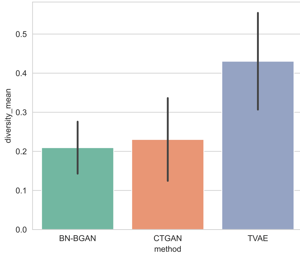
Data Diversity Higher is Better
