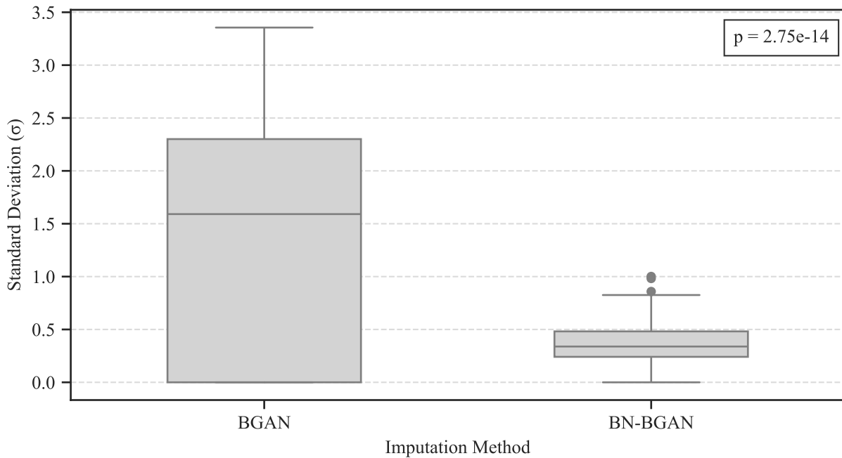
Comparison of Imputation Uncertainty
