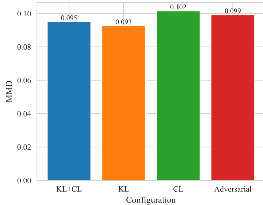
Loss Configurations: MMD
