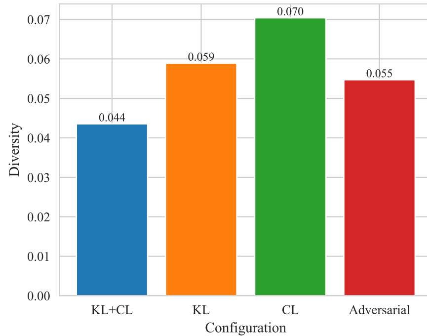
Loss Configurations: Diversity
