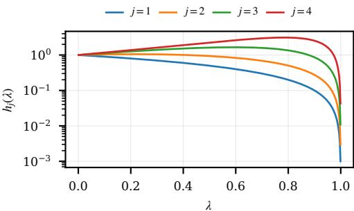
(a) Scale functions h_j
