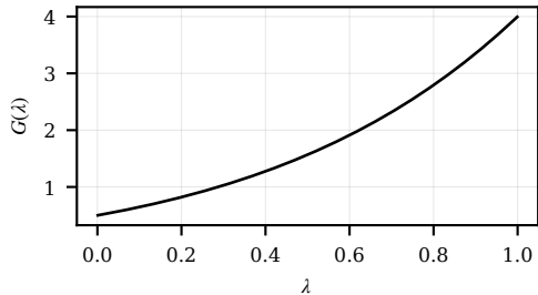
(b) Three-scale ratio G(\lambda)
