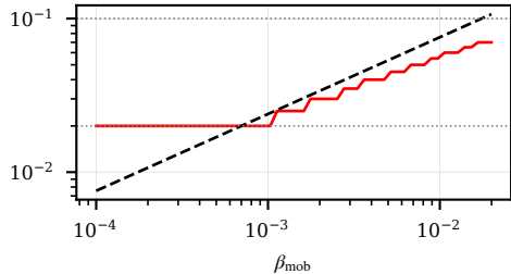
(b) Square-root law
