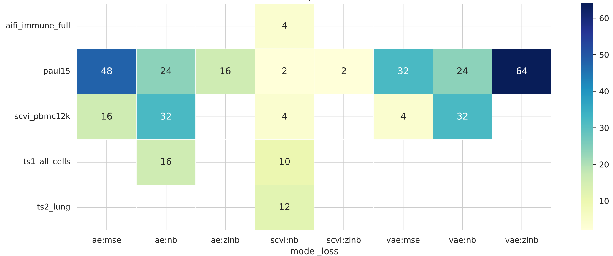
Best Latent Dimension per Dataset × Model/Loss
