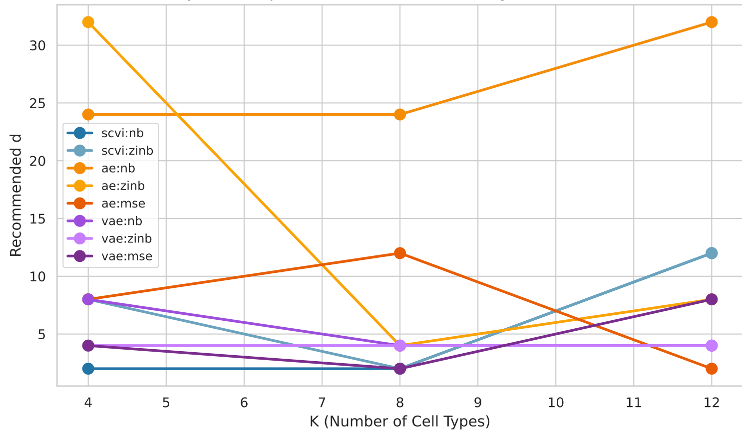
Splatter: Optimal d vs K (Controlled Synthetic Data)
