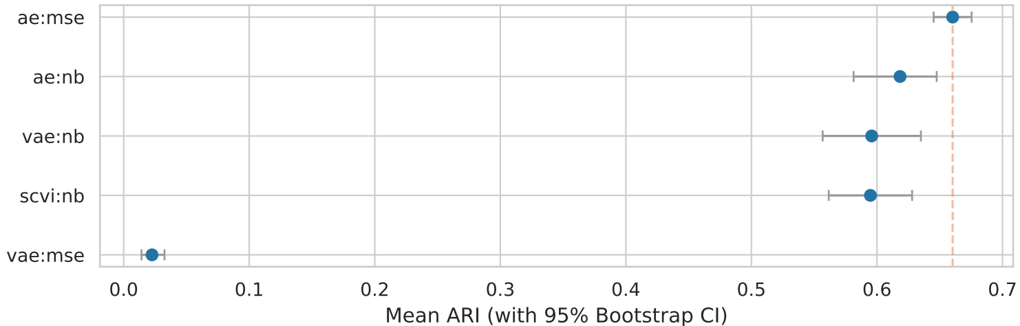
Model Performance — PBMC12k
