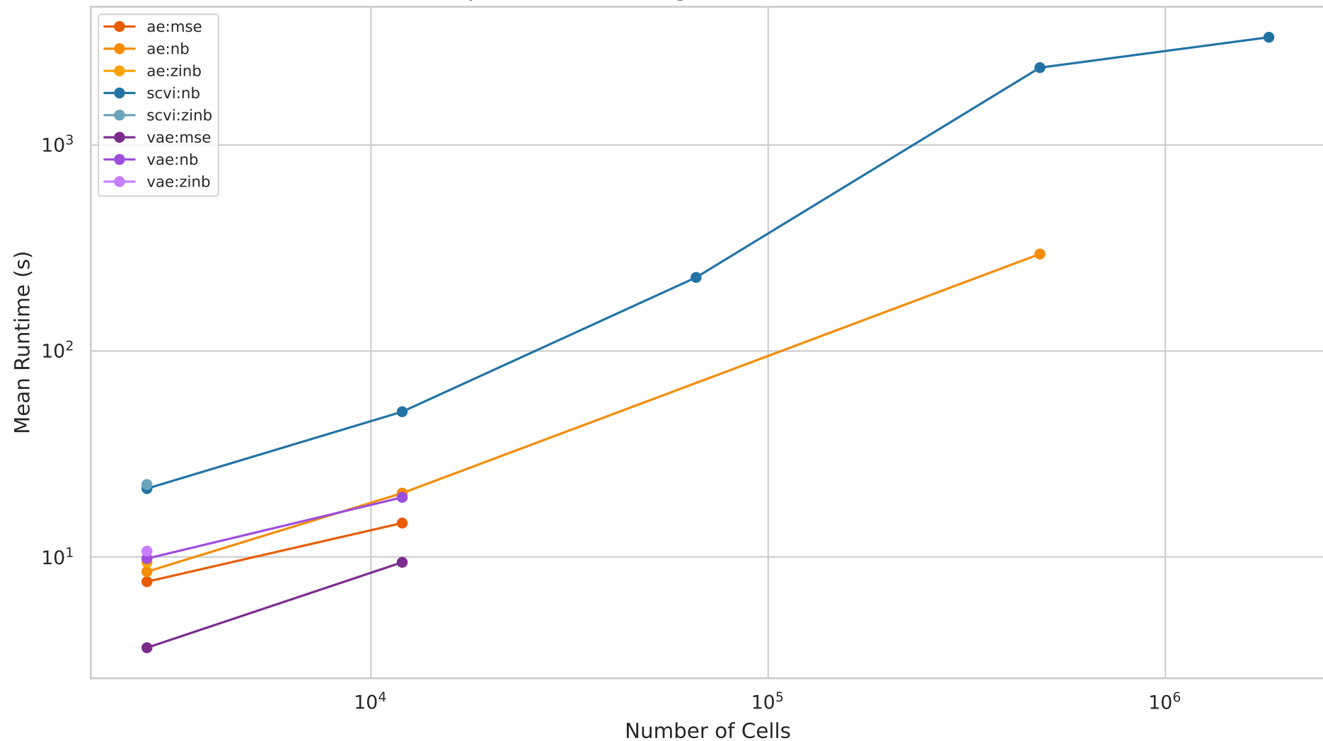
Computational Scaling: Runtime vs Dataset Size
