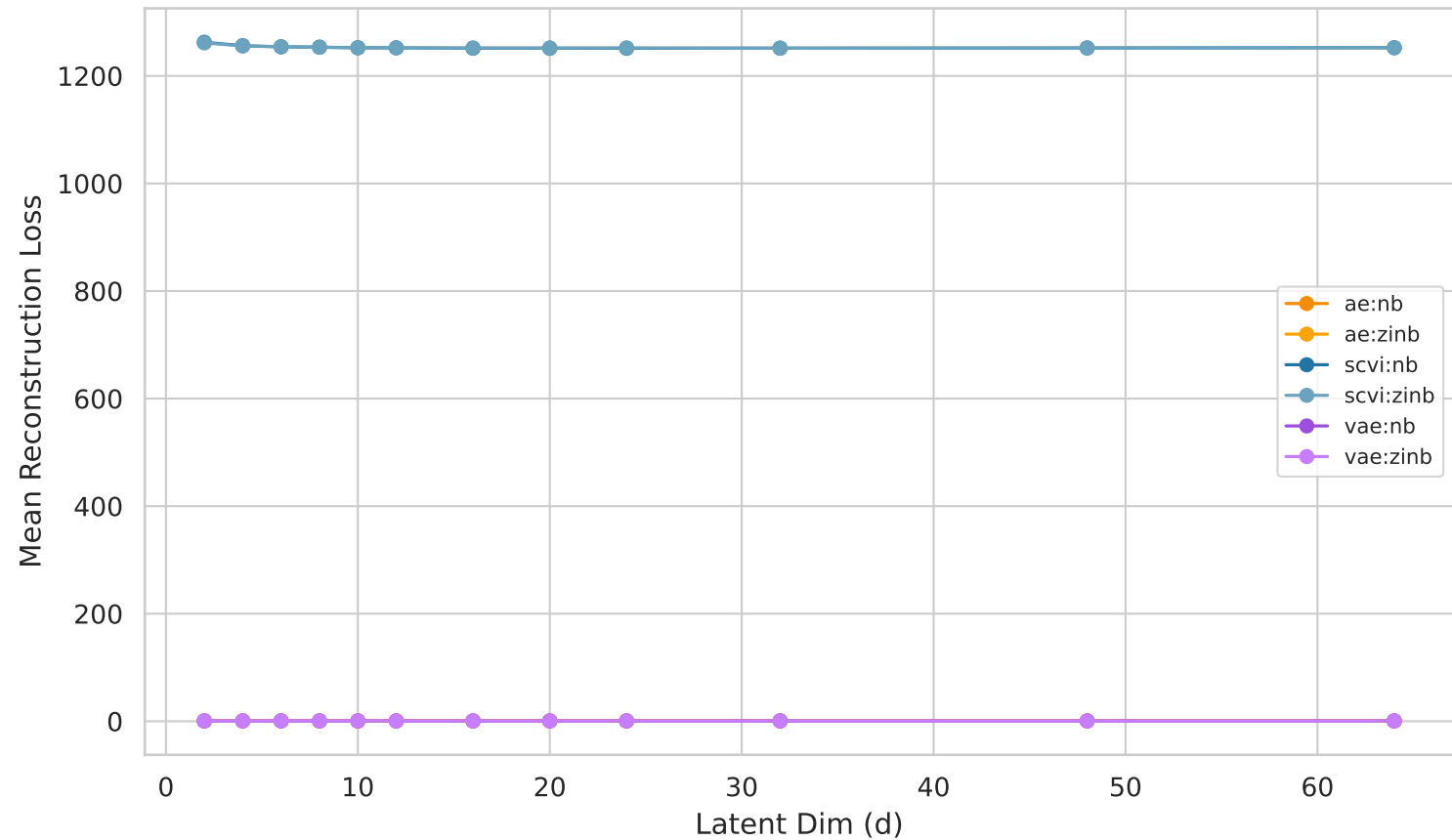
Reconstruction Loss — Paul15
