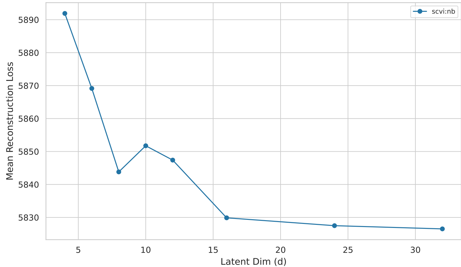
Reconstruction Loss — TS2 Lung
