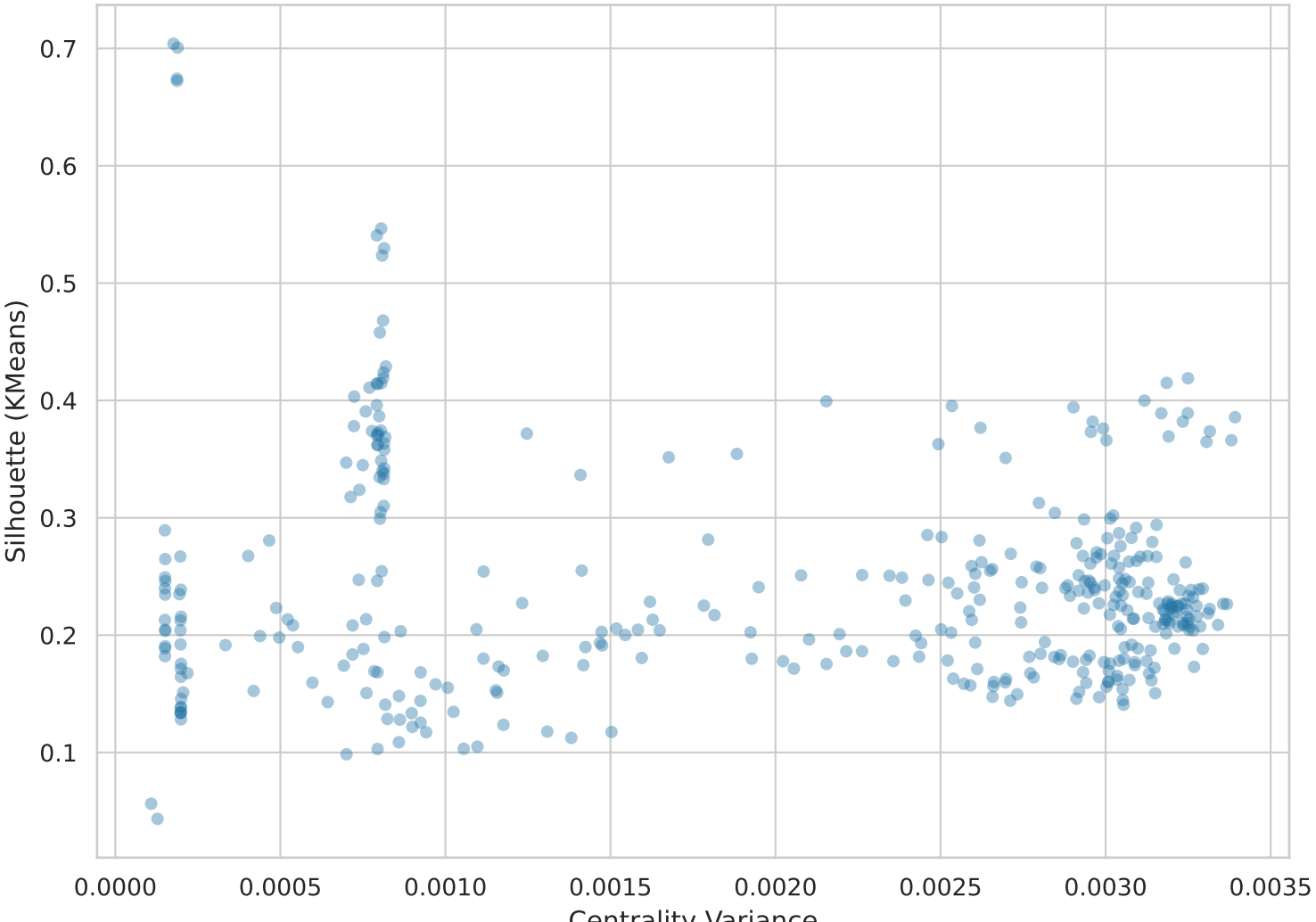
Centrality vs Silhouette ( r=0.050 )
